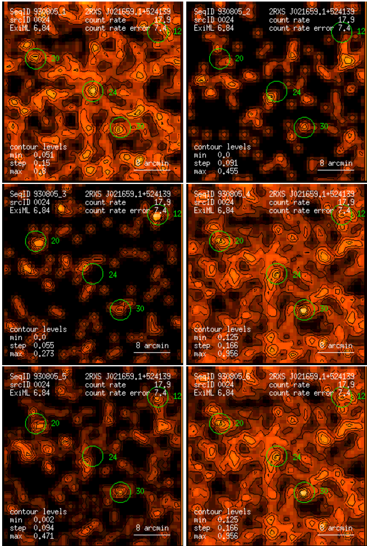
Figure 24: RASS 930805: detection 0024: band rate images, Gaussian filter: (1) PSPC channels 11 – 41, (2) 52 – 90, (3) 91 – 201, (4) 11 – 235, (5) 52 – 201, (6) 11 – 201. Broad band rates in counts/ks. Band rate contour levels in counts/ks/arcmin 2 .
