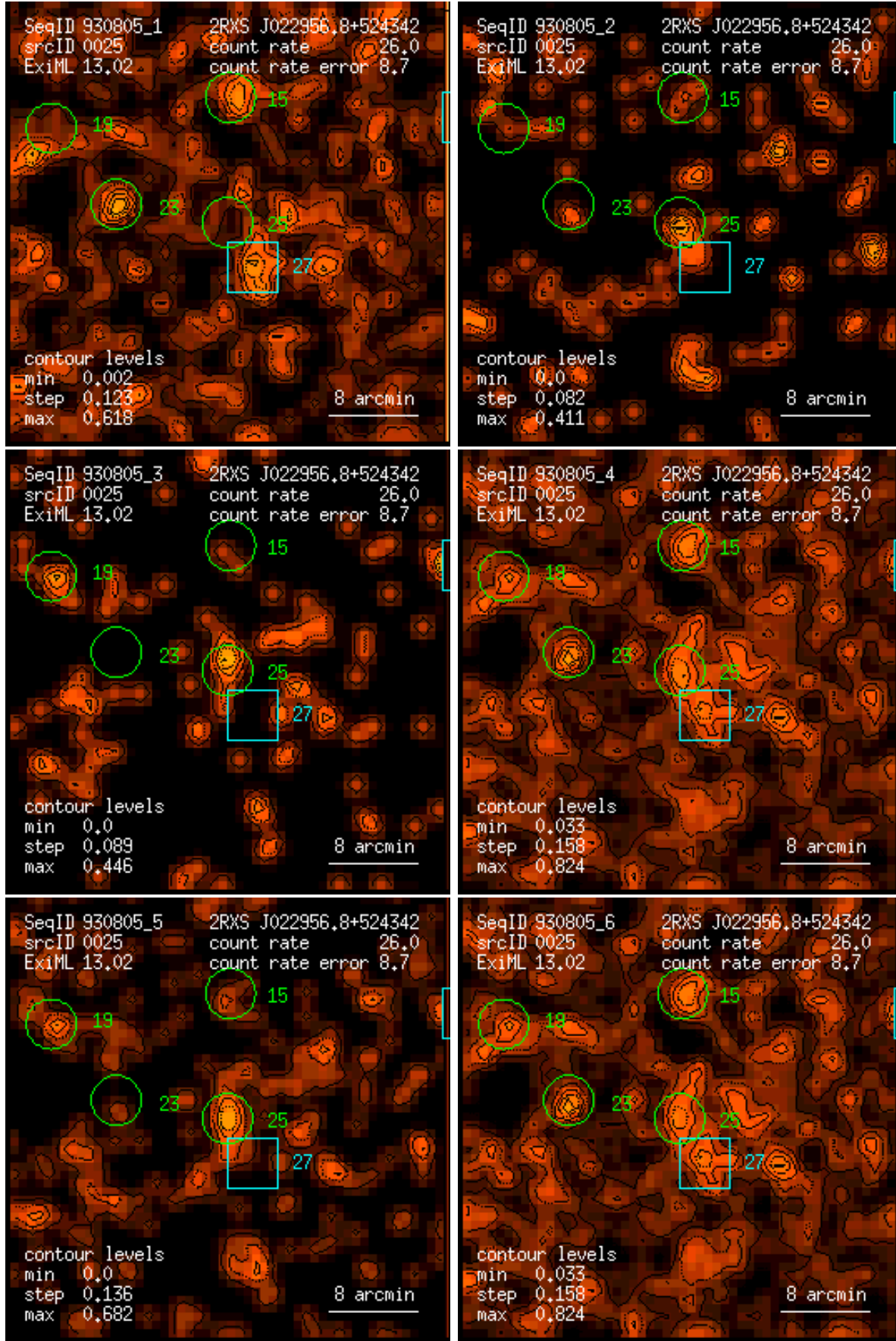
Figure 25: RASS 930805: detection 0025: band rate images, Gaussian filter: (1) PSPC channels 11 – 41, (2) 52 – 90, (3) 91 – 201, (4) 11 – 235, (5) 52 – 201, (6) 11 – 201. Broad band rates in counts/ks. Band rate contour levels in counts/ks/arcmin 2 .
