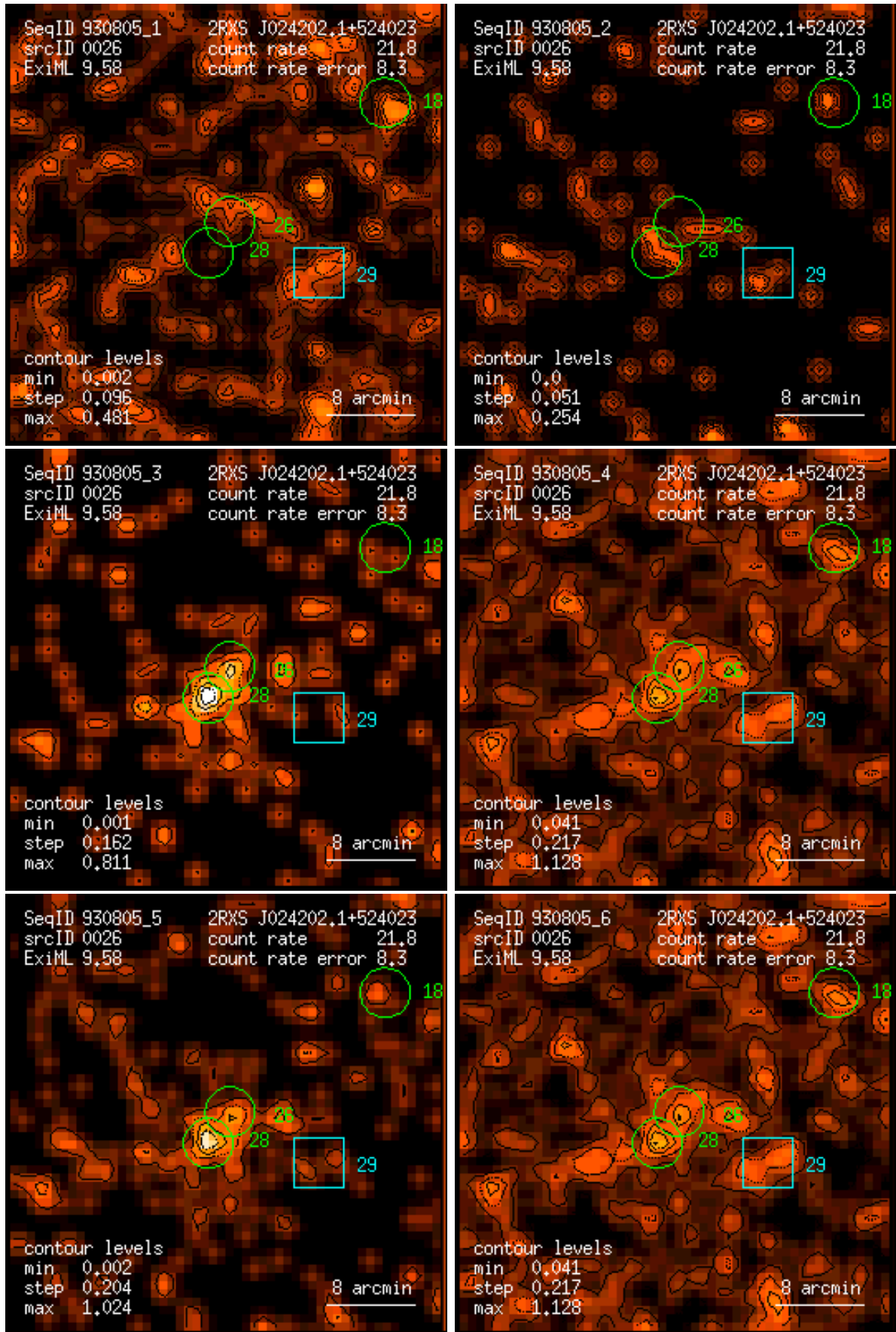
Figure 26: RASS 930805: detection 0026: band rate images, Gaussian filter: (1) PSPC channels 11 – 41, (2) 52 – 90, (3) 91 – 201, (4) 11 – 235, (5) 52 – 201, (6) 11 – 201. Broad band rates in counts/ks. Band rate contour levels in counts/ks/arcmin 2 .
