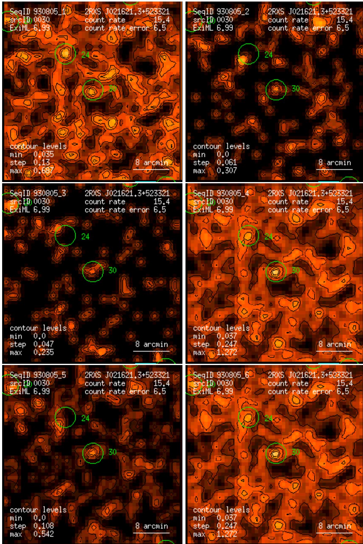
Figure 30: RASS 930805: detection 0030: band rate images, Gaussian filter: (1) PSPC channels 11 – 41, (2) 52 – 90, (3) 91 – 201, (4) 11 – 235, (5) 52 – 201, (6) 11 – 201. Broad band rates in counts/ks. Band rate contour levels in counts/ks/arcmin 2 .
