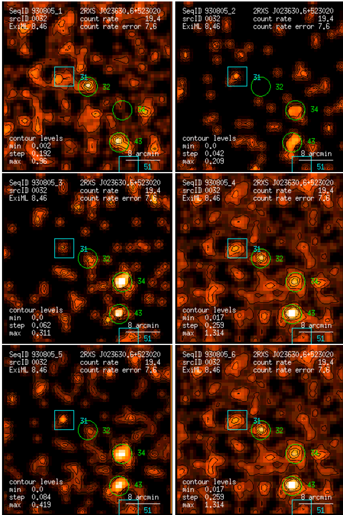
Figure 32: RASS 930805: detection 0032: band rate images, Gaussian filter: (1) PSPC channels 11 – 41, (2) 52 – 90, (3) 91 – 201, (4) 11 – 235, (5) 52 – 201, (6) 11 – 201. Broad band rates in counts/ks. Band rate contour levels in counts/ks/arcmin 2 .
