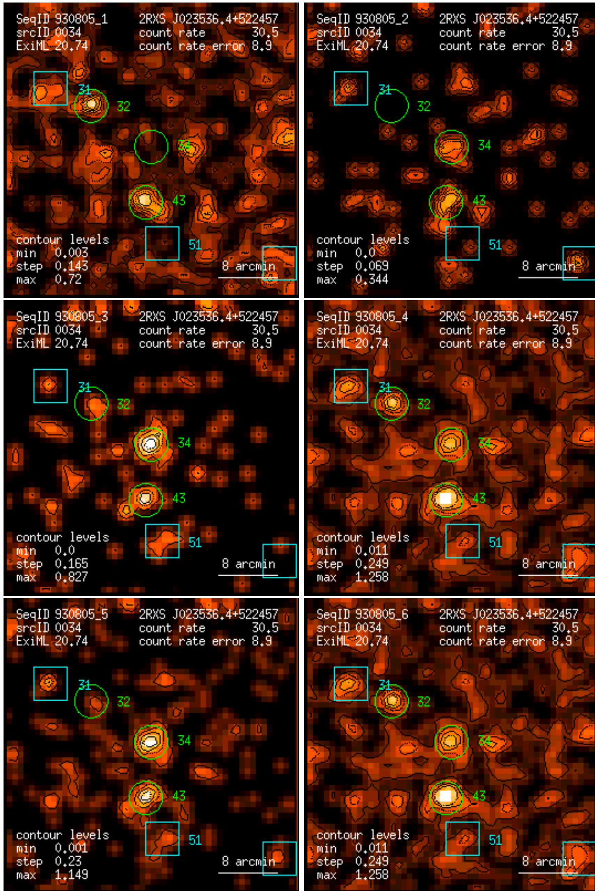
Figure 34: RASS 930805: detection 0034: band rate images, Gaussian filter: (1) PSPC channels 11 – 41, (2) 52 – 90, (3) 91 – 201, (4) 11 – 235, (5) 52 – 201, (6) 11 – 201. Broad band rates in counts/ks. Band rate contour levels in counts/ks/arcmin 2 .
