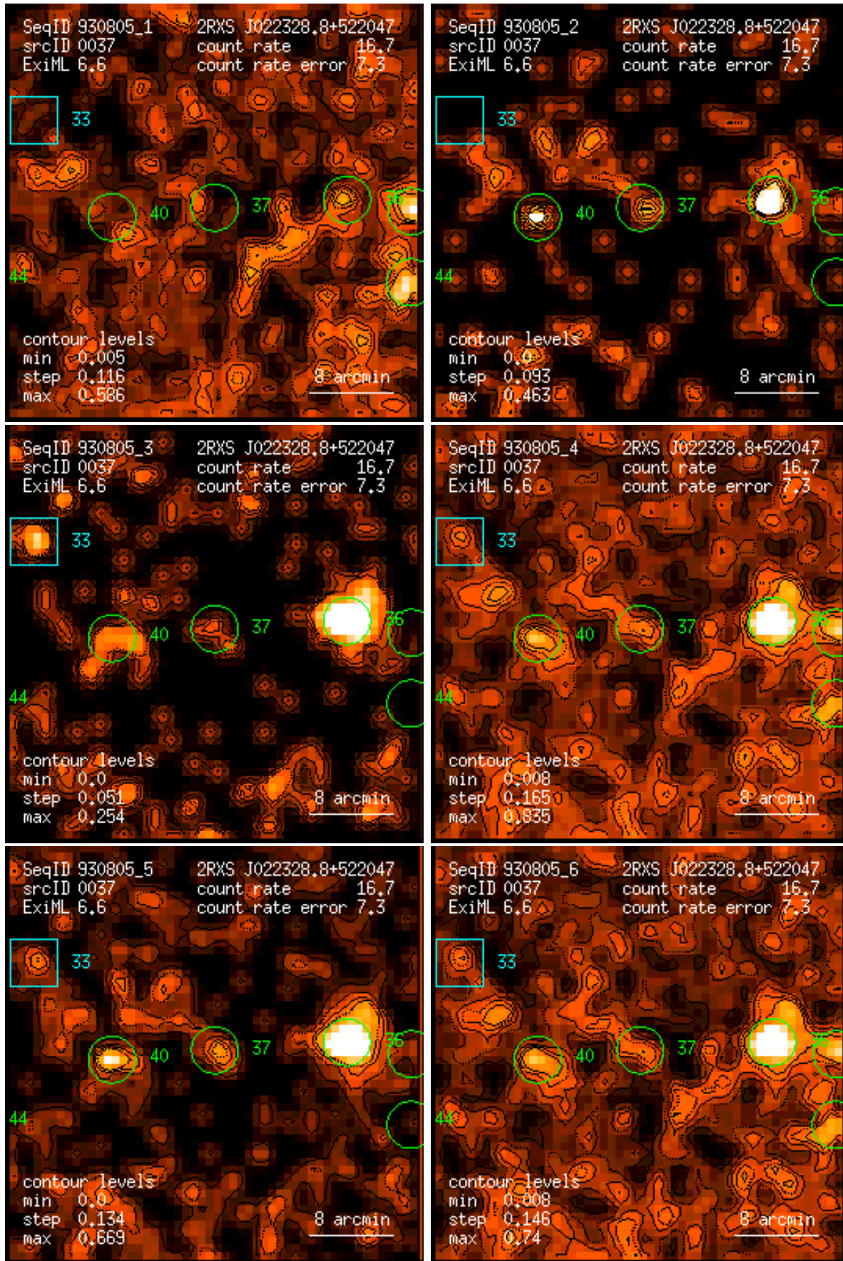
Figure 37: RASS 930805: detection 0037: band rate images, Gaussian filter: (1) PSPC channels 11 – 41, (2) 52 – 90, (3) 91 – 201, (4) 11 – 235, (5) 52 – 201, (6) 11 – 201. Broad band rates in counts/ks. Band rate contour levels in counts/ks/arcmin 2 .
