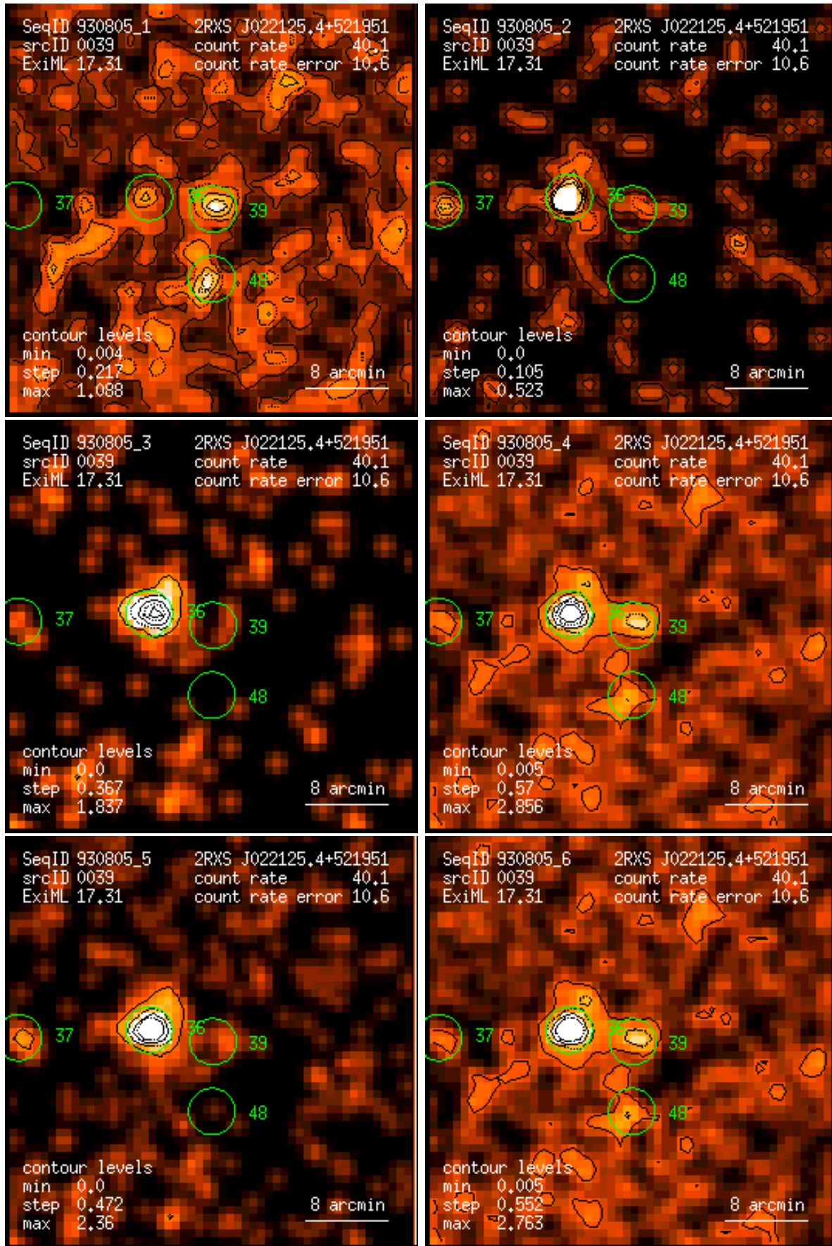
Figure 39: RASS 930805: detection 0039: band rate images, Gaussian filter: (1) PSPC channels 11 – 41, (2) 52 – 90, (3) 91 – 201, (4) 11 – 235, (5) 52 – 201, (6) 11 – 201. Broad band rates in counts/ks. Band rate contour levels in counts/ks/arcmin 2 .
