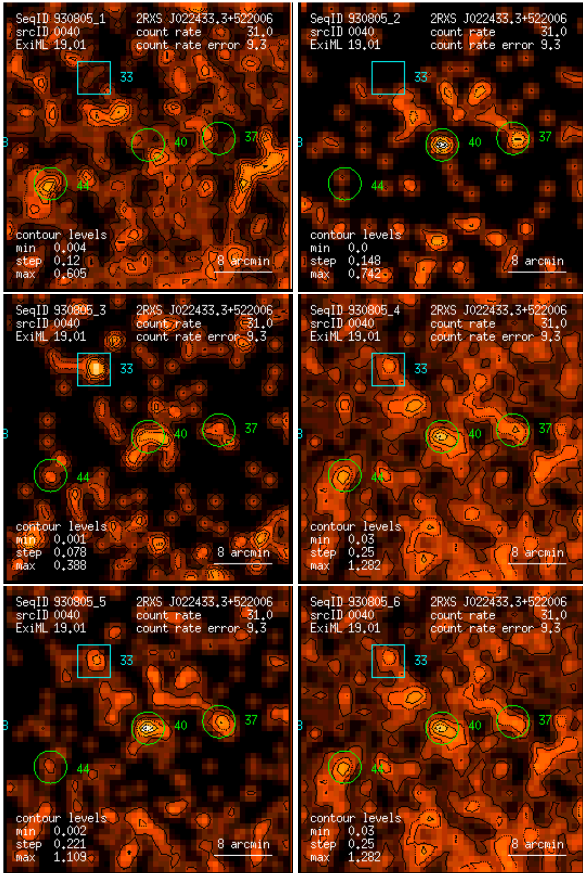
Figure 40: RASS 930805: detection 0040: band rate images, Gaussian filter: (1) PSPC channels 11 – 41, (2) 52 – 90, (3) 91 – 201, (4) 11 – 235, (5) 52 – 201, (6) 11 – 201. Broad band rates in counts/ks. Band rate contour levels in counts/ks/arcmin 2 .
