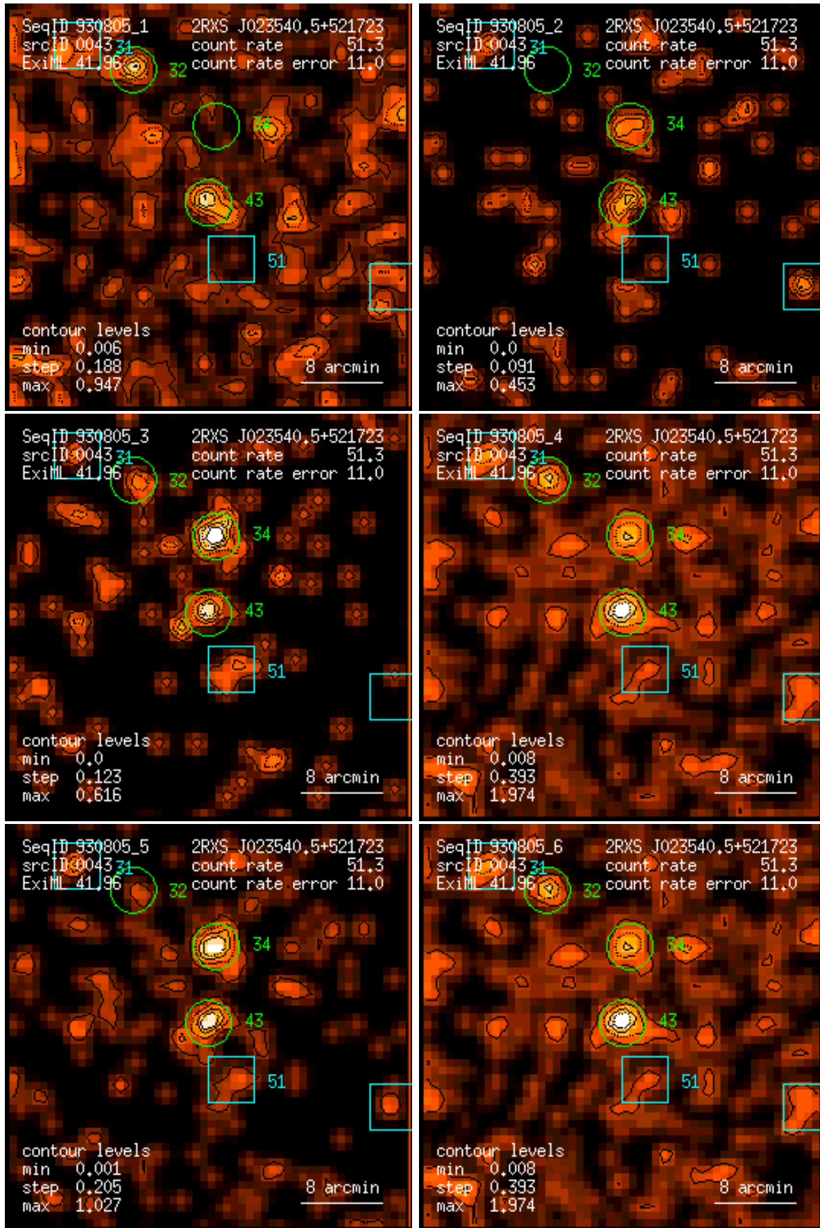
Figure 43: RASS 930805: detection 0043: band rate images, Gaussian filter: (1) PSPC channels 11 – 41, (2) 52 – 90, (3) 91 – 201, (4) 11 – 235, (5) 52 – 201, (6) 11 – 201. Broad band rates in counts/ks. Band rate contour levels in counts/ks/arcmin 2 .
