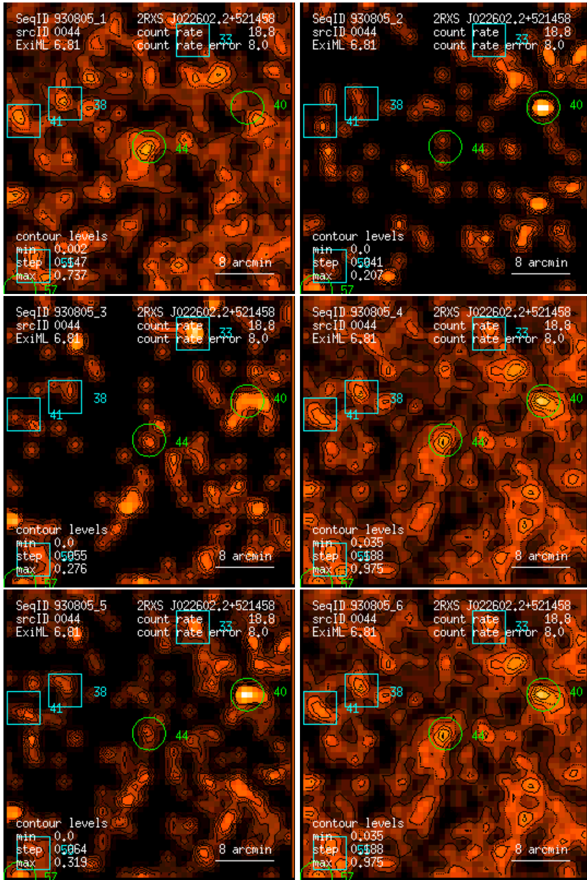
Figure 44: RASS 930805: detection 0044: band rate images, Gaussian filter: (1) PSPC channels 11 – 41, (2) 52 – 90, (3) 91 – 201, (4) 11 – 235, (5) 52 – 201, (6) 11 – 201. Broad band rates in counts/ks. Band rate contour levels in counts/ks/arcmin 2 .
