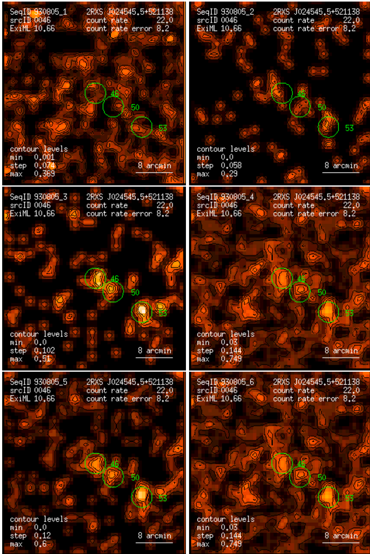
Figure 46: RASS 930805: detection 0046: band rate images, Gaussian filter: (1) PSPC channels 11 – 41, (2) 52 – 90, (3) 91 – 201, (4) 11 – 235, (5) 52 – 201, (6) 11 – 201. Broad band rates in counts/ks. Band rate contour levels in counts/ks/arcmin 2 .
