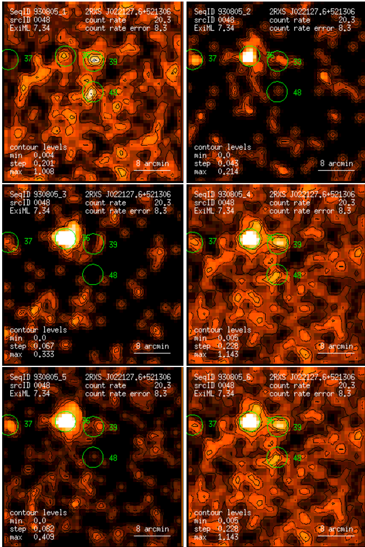
Figure 48: RASS 930805: detection 0048: band rate images, Gaussian filter: (1) PSPC channels 11 – 41, (2) 52 – 90, (3) 91 – 201, (4) 11 – 235, (5) 52 – 201, (6) 11 – 201. Broad band rates in counts/ks. Band rate contour levels in counts/ks/arcmin 2 .
