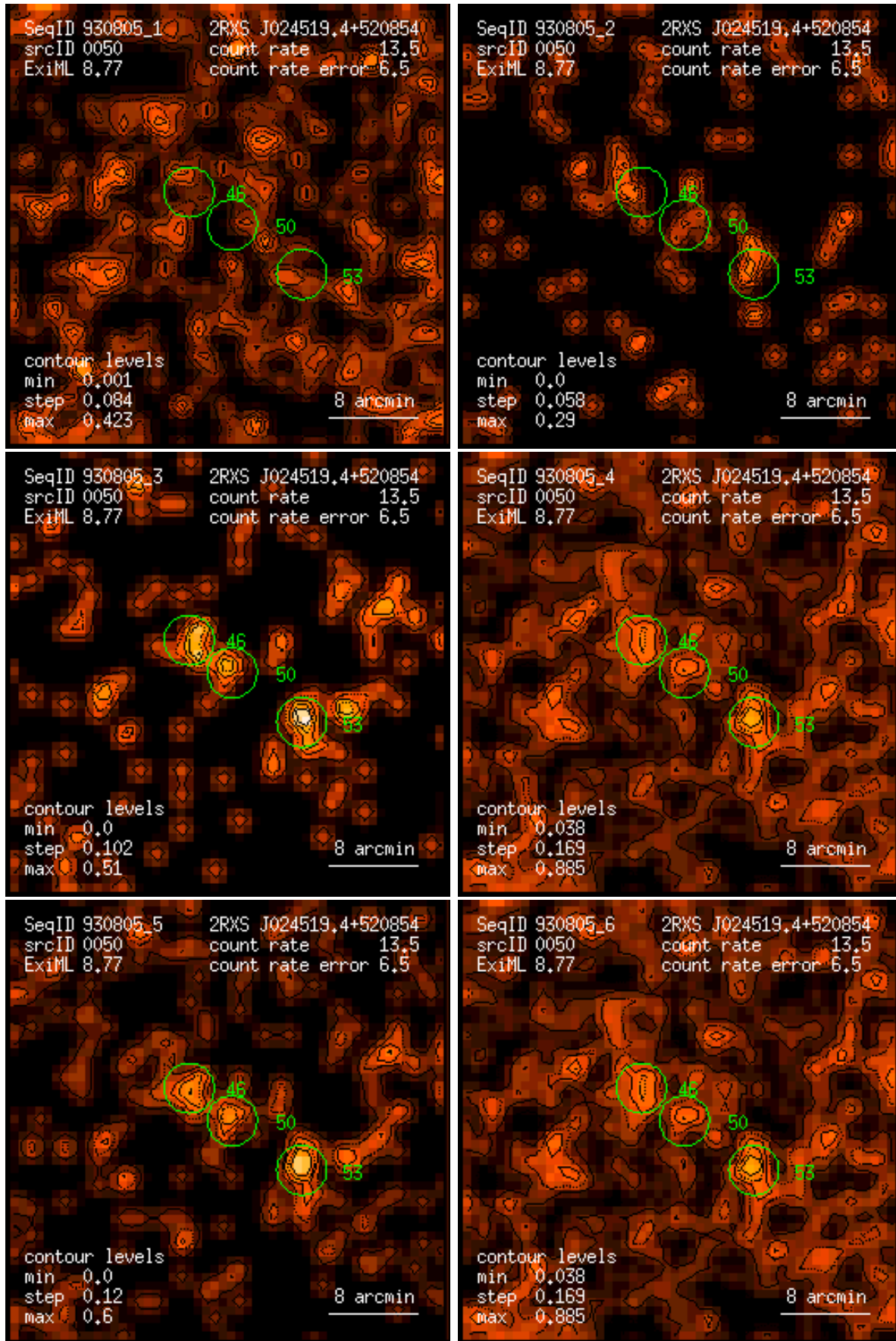
Figure 50: RASS 930805: detection 0050: band rate images, Gaussian filter: (1) PSPC channels 11 – 41, (2) 52 – 90, (3) 91 – 201, (4) 11 – 235, (5) 52 – 201, (6) 11 – 201. Broad band rates in counts/ks. Band rate contour levels in counts/ks/arcmin 2 .
