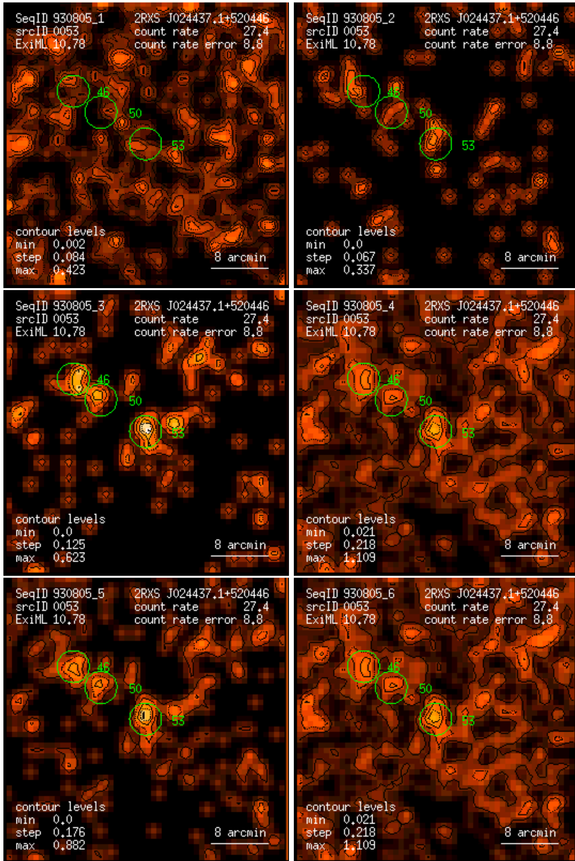
Figure 53: RASS 930805: detection 0053: band rate images, Gaussian filter: (1) PSPC channels 11 – 41, (2) 52 – 90, (3) 91 – 201, (4) 11 – 235, (5) 52 – 201, (6) 11 – 201. Broad band rates in counts/ks. Band rate contour levels in counts/ks/arcmin 2 .
