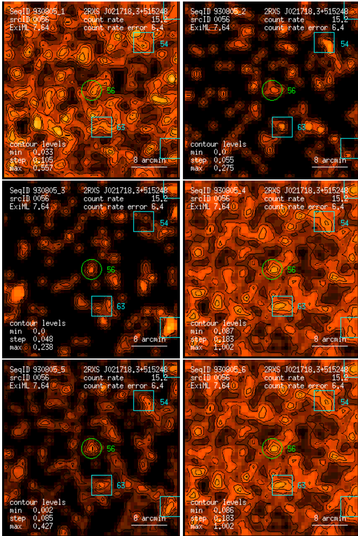
Figure 56: RASS 930805: detection 0056: band rate images, Gaussian filter: (1) PSPC channels 11 – 41, (2) 52 – 90, (3) 91 – 201, (4) 11 – 235, (5) 52 – 201, (6) 11 – 201. Broad band rates in counts/ks. Band rate contour levels in counts/ks/arcmin 2 .
