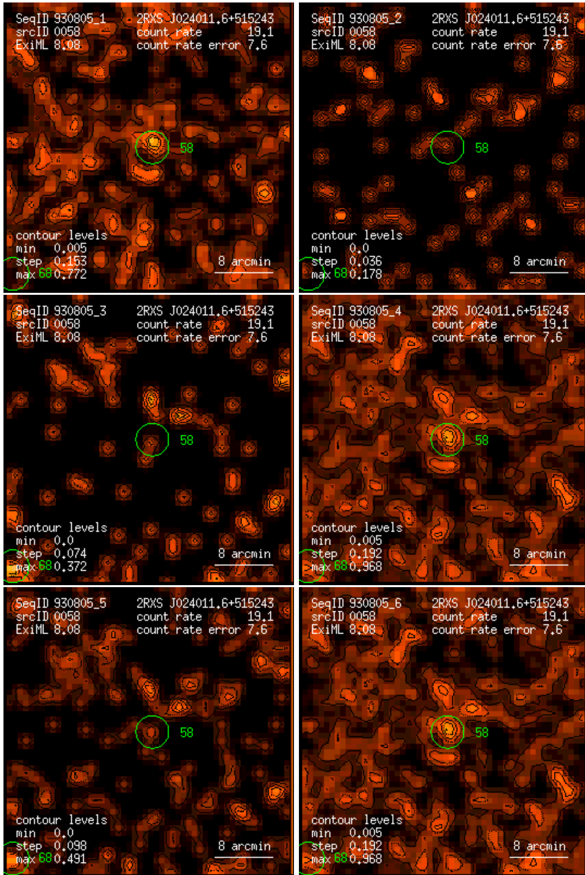
Figure 58: RASS 930805: detection 0058: band rate images, Gaussian filter: (1) PSPC channels 11 – 41, (2) 52 – 90, (3) 91 – 201, (4) 11 – 235, (5) 52 – 201, (6) 11 – 201. Broad band rates in counts/ks. Band rate contour levels in counts/ks/arcmin 2 .
