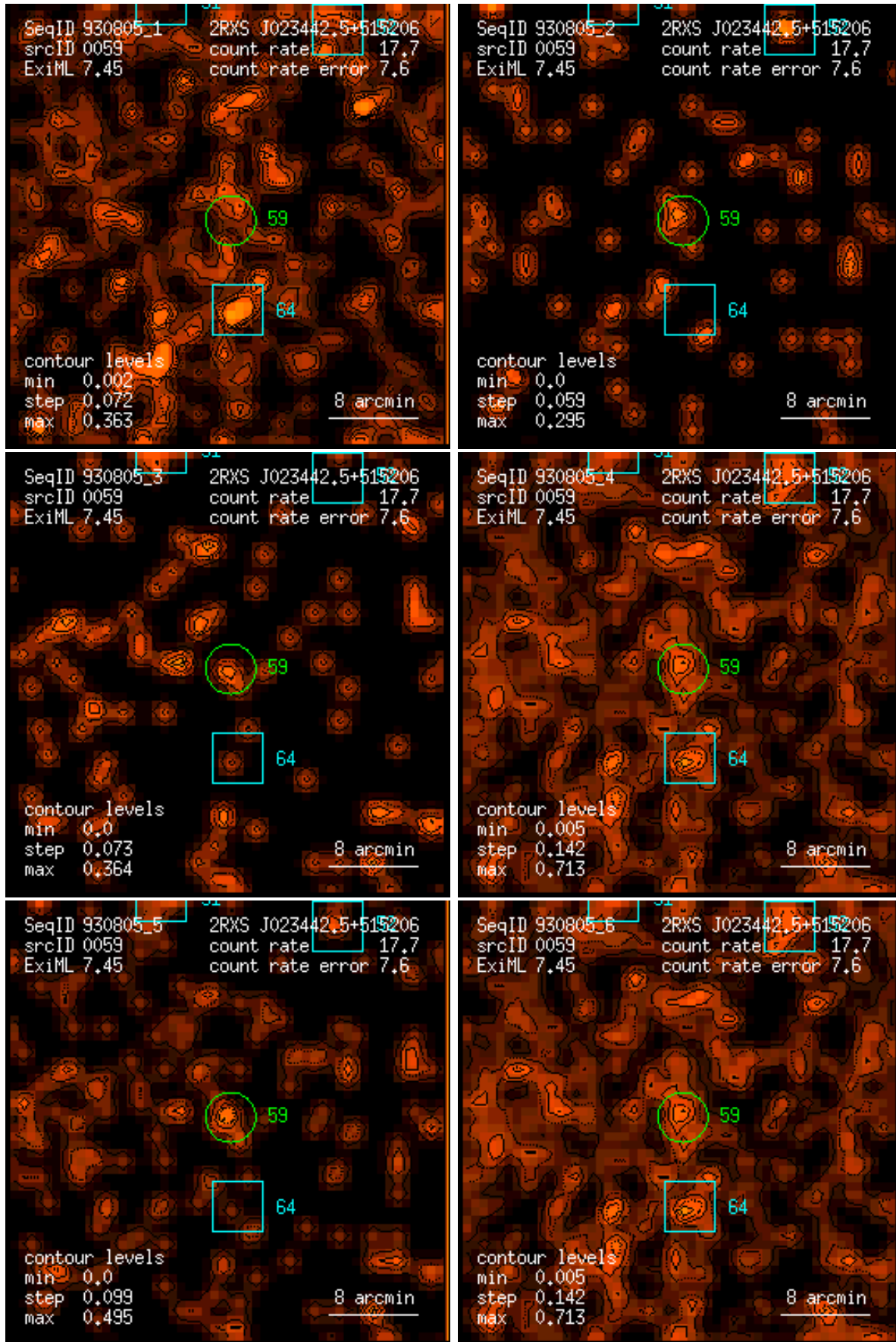
Figure 59: RASS 930805: detection 0059: band rate images, Gaussian filter: (1) PSPC channels 11 – 41, (2) 52 – 90, (3) 91 – 201, (4) 11 – 235, (5) 52 – 201, (6) 11 – 201. Broad band rates in counts/ks. Band rate contour levels in counts/ks/arcmin 2 .
