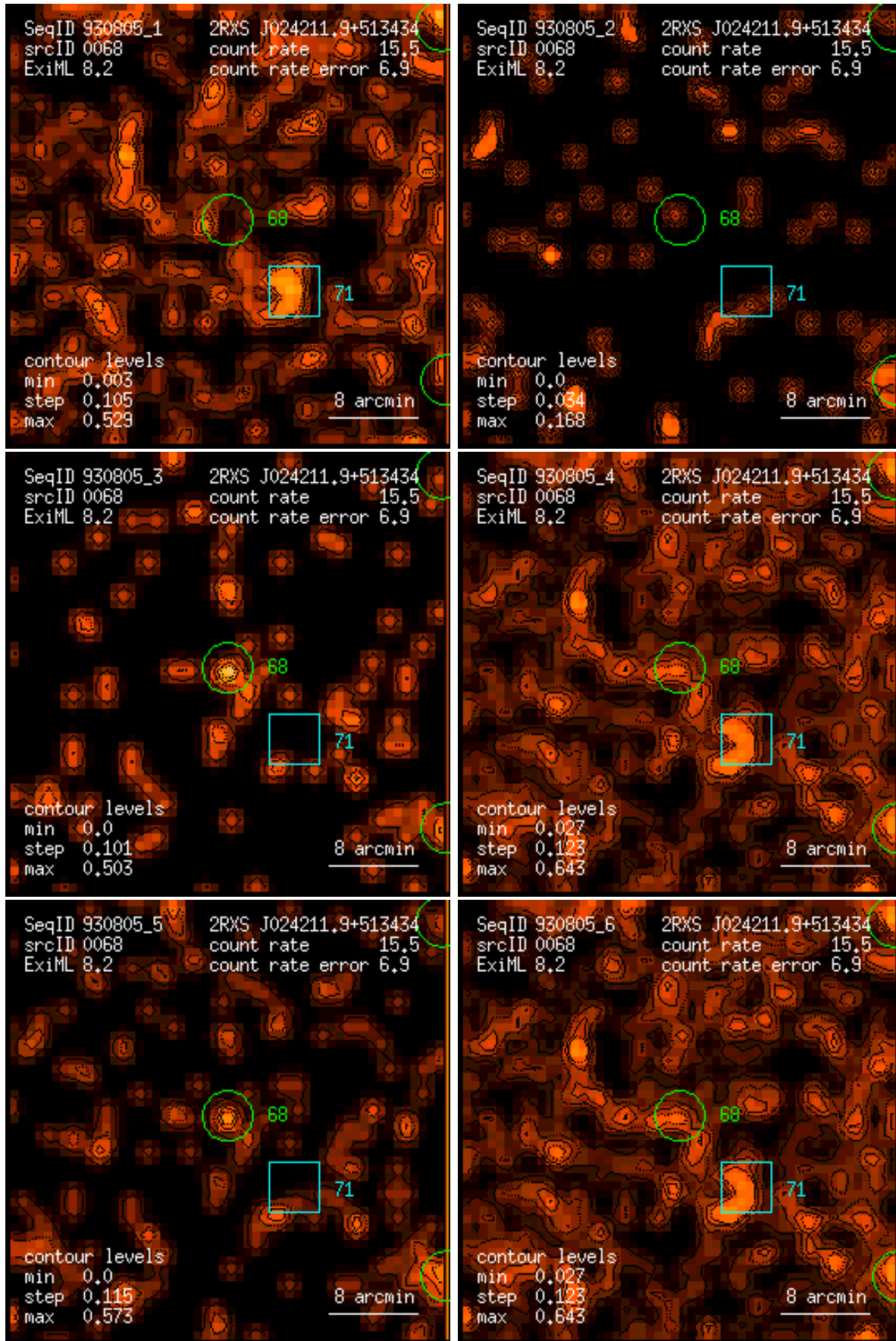
Figure 68: RASS 930805: detection 0068: band rate images, Gaussian filter: (1) PSPC channels 11 – 41, (2) 52 – 90, (3) 91 – 201, (4) 11 – 235, (5) 52 – 201, (6) 11 – 201. Broad band rates in counts/ks. Band rate contour levels in counts/ks/arcmin 2 .
