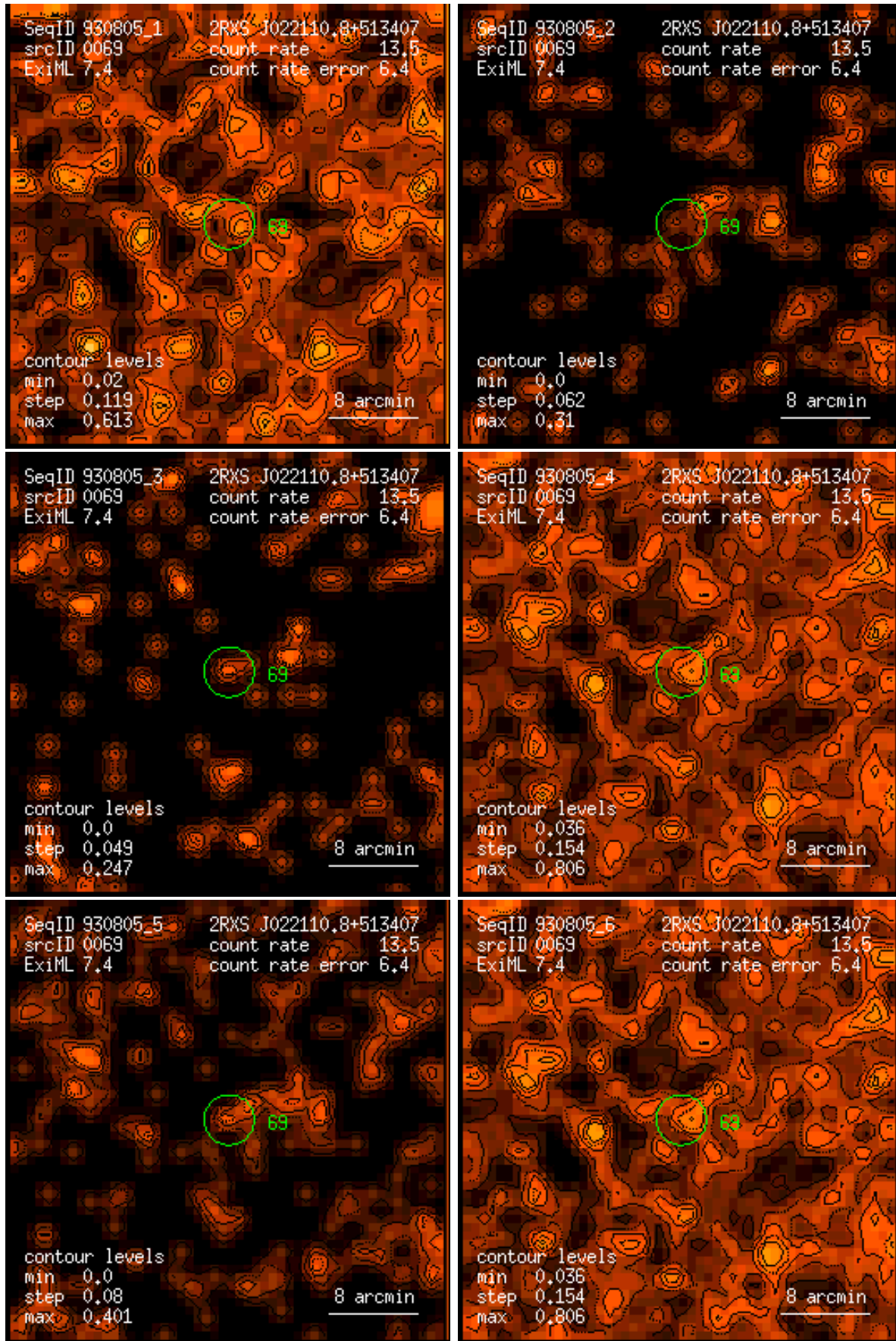
Figure 69: RASS 930805: detection 0069: band rate images, Gaussian filter: (1) PSPC channels 11 – 41, (2) 52 – 90, (3) 91 – 201, (4) 11 – 235, (5) 52 – 201, (6) 11 – 201. Broad band rates in counts/ks. Band rate contour levels in counts/ks/arcmin 2 .
