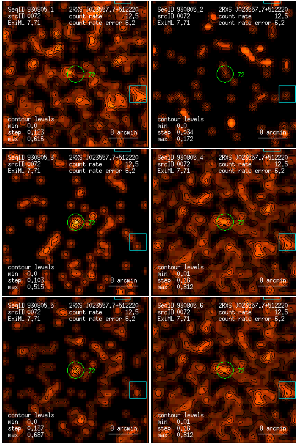
Figure 72: RASS 930805: detection 0072: band rate images, Gaussian filter: (1) PSPC channels 11 – 41, (2) 52 – 90, (3) 91 – 201, (4) 11 – 235, (5) 52 – 201, (6) 11 – 201. Broad band rates in counts/ks. Band rate contour levels in counts/ks/arcmin 2 .
