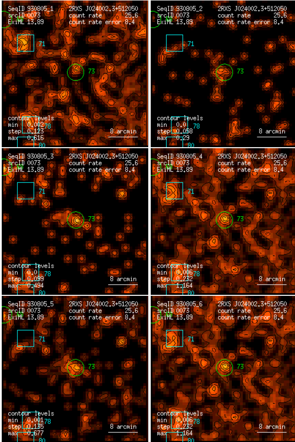
Figure 73: RASS 930805: detection 0073: band rate images, Gaussian filter: (1) PSPC channels 11 – 41, (2) 52 – 90, (3) 91 – 201, (4) 11 – 235, (5) 52 – 201, (6) 11 – 201. Broad band rates in counts/ks. Band rate contour levels in counts/ks/arcmin 2 .
