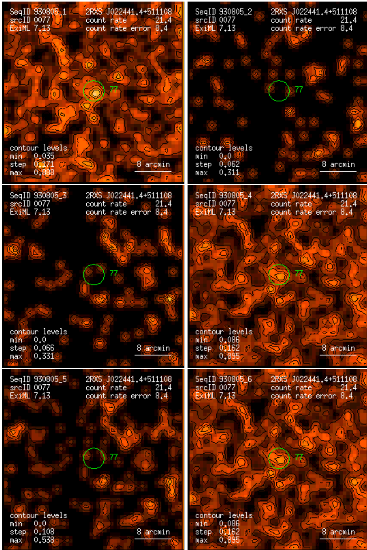
Figure 77: RASS 930805: detection 0077: band rate images, Gaussian filter: (1) PSPC channels 11 – 41, (2) 52 – 90, (3) 91 – 201, (4) 11 – 235, (5) 52 – 201, (6) 11 – 201. Broad band rates in counts/ks. Band rate contour levels in counts/ks/arcmin 2 .
