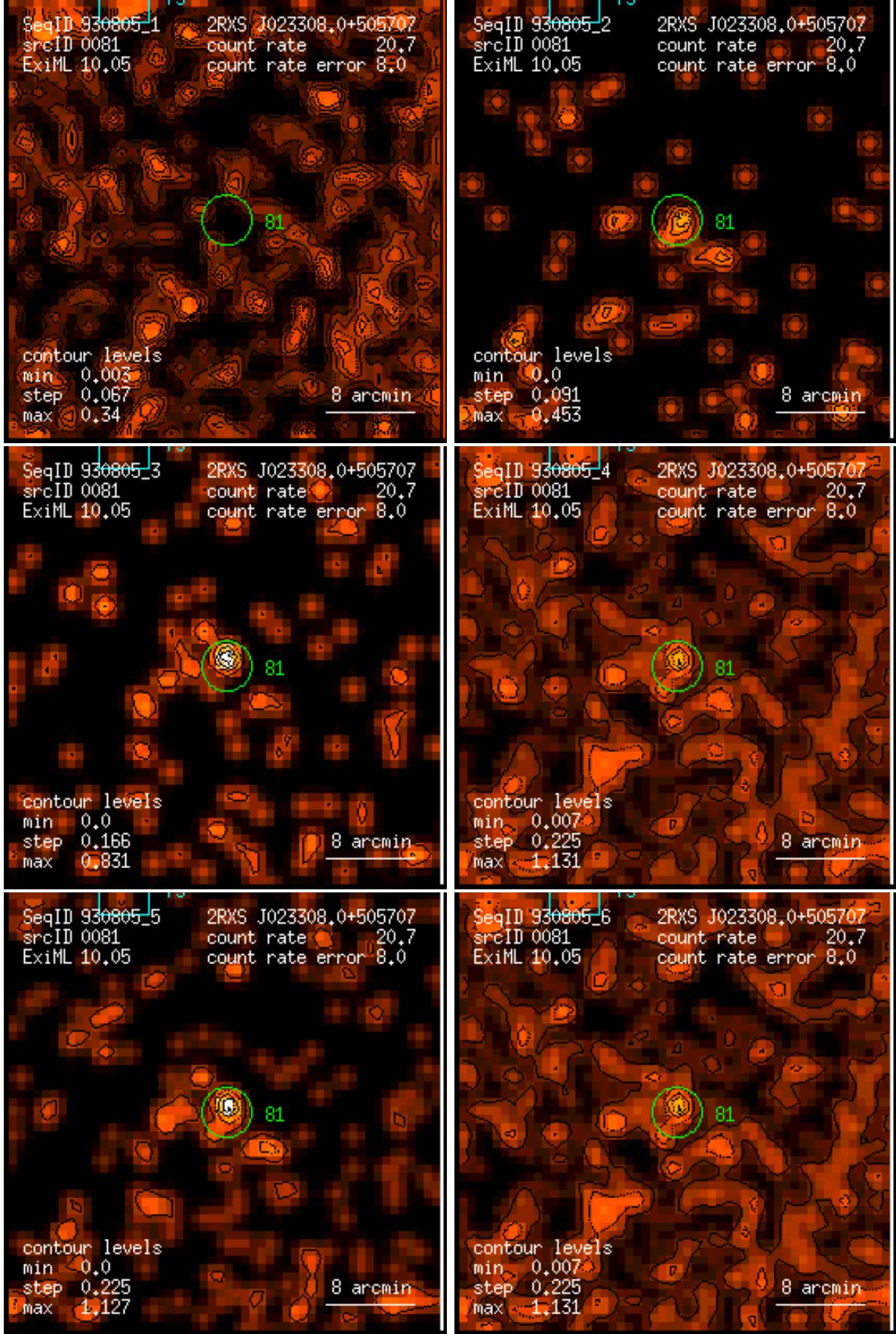
Figure 81: RASS 930805: detection 0081: band rate images, Gaussian filter: (1) PSPC channels 11 – 41, (2) 52 – 90, (3) 91 – 201, (4) 11 – 235, (5) 52 – 201, (6) 11 – 201. Broad band rates in counts/ks. Band rate contour levels in counts/ks/arcmin 2 .
