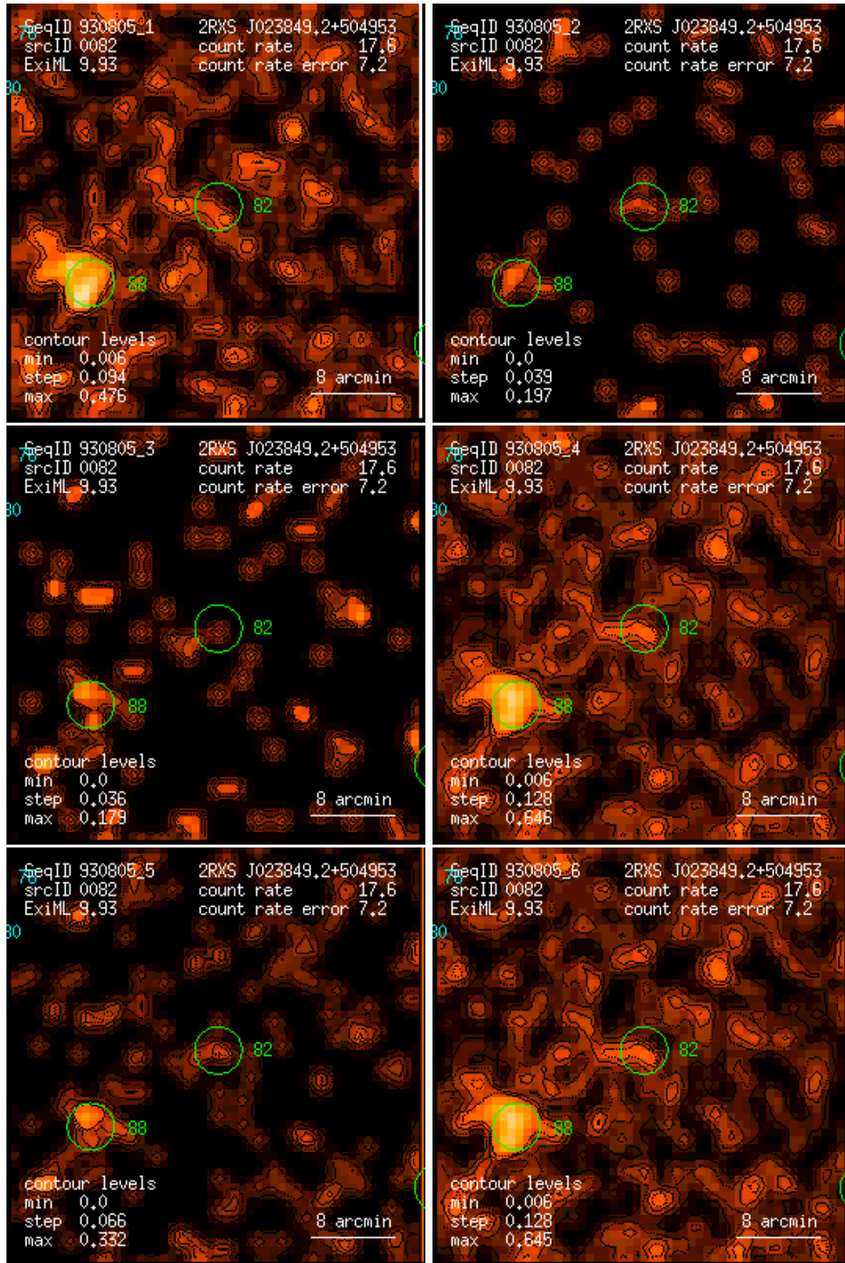
Figure 82: RASS 930805: detection 0082: band rate images, Gaussian filter: (1) PSPC channels 11 – 41, (2) 52 – 90, (3) 91 – 201, (4) 11 – 235, (5) 52 – 201, (6) 11 – 201. Broad band rates in counts/ks. Band rate contour levels in counts/ks/arcmin 2 .
