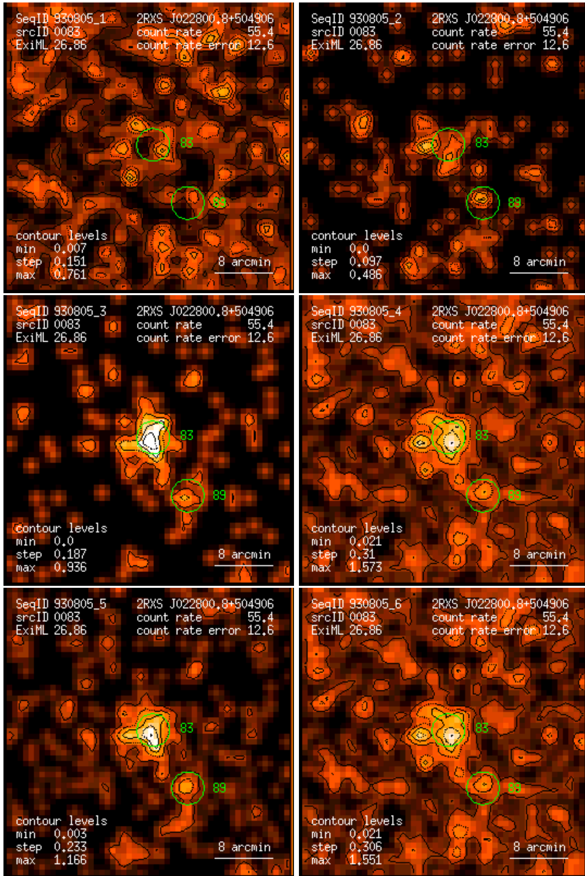
Figure 83: RASS 930805: detection 0083: band rate images, Gaussian filter: (1) PSPC channels 11 – 41, (2) 52 – 90, (3) 91 – 201, (4) 11 – 235, (5) 52 – 201, (6) 11 – 201. Broad band rates in counts/ks. Band rate contour levels in counts/ks/arcmin 2 .
