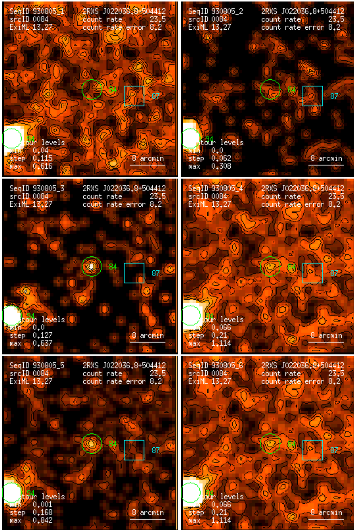
Figure 84: RASS 930805: detection 0084: band rate images, Gaussian filter: (1) PSPC channels 11 – 41, (2) 52 – 90, (3) 91 – 201, (4) 11 – 235, (5) 52 – 201, (6) 11 – 201. Broad band rates in counts/ks. Band rate contour levels in counts/ks/arcmin 2 .
