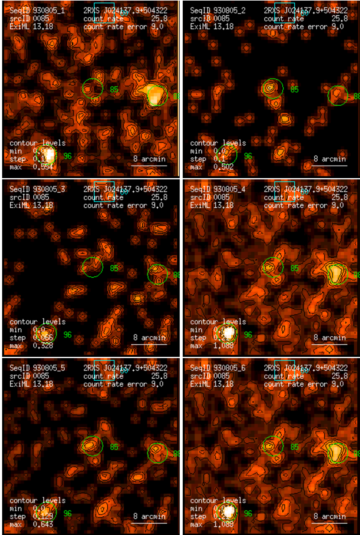
Figure 85: RASS 930805: detection 0085: band rate images, Gaussian filter: (1) PSPC channels 11 – 41, (2) 52 – 90, (3) 91 – 201, (4) 11 – 235, (5) 52 – 201, (6) 11 – 201. Broad band rates in counts/ks. Band rate contour levels in counts/ks/arcmin 2 .
