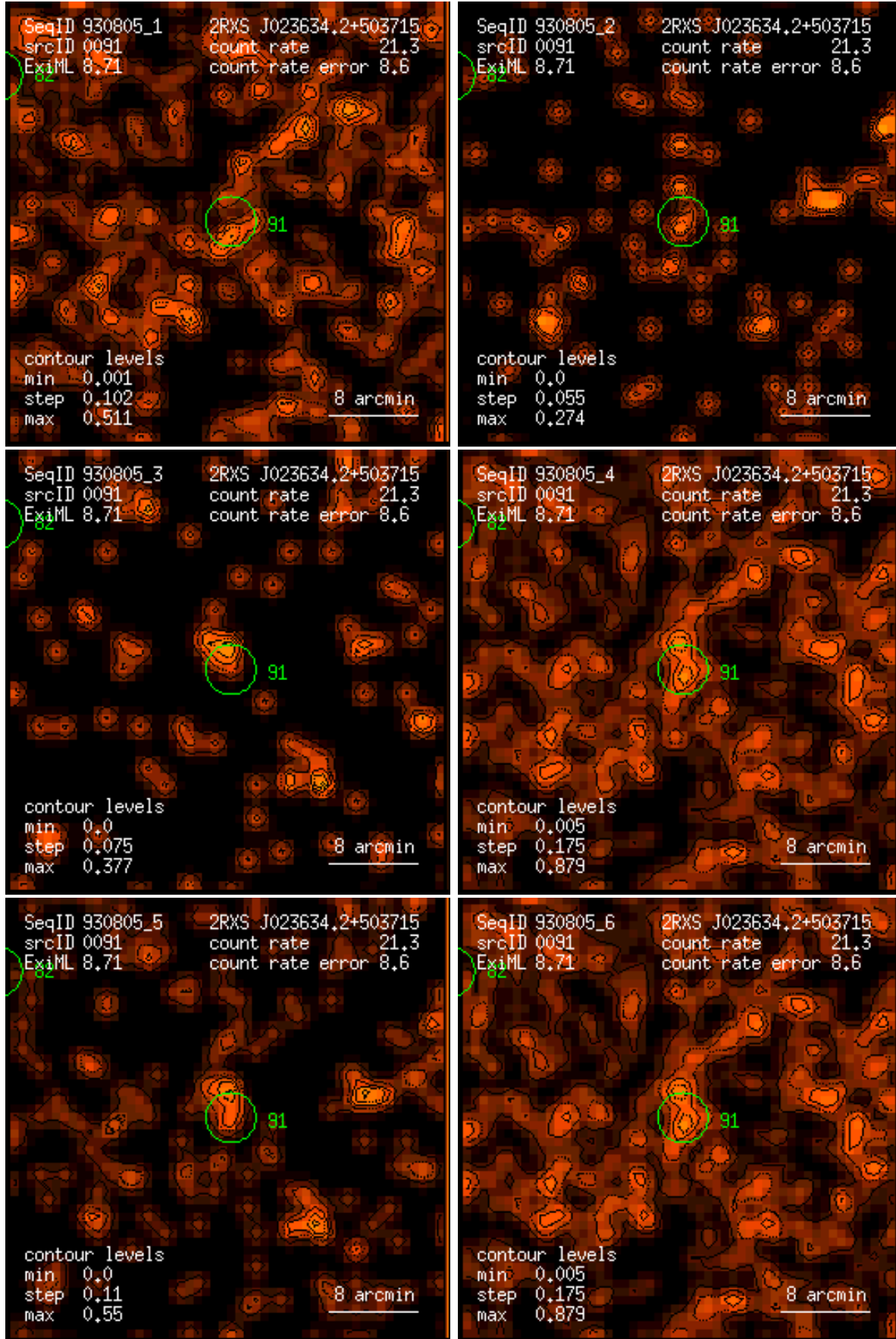
Figure 91: RASS 930805: detection 0091: band rate images, Gaussian filter: (1) PSPC channels 11 – 41, (2) 52 – 90, (3) 91 – 201, (4) 11 – 235, (5) 52 – 201, (6) 11 – 201. Broad band rates in counts/ks. Band rate contour levels in counts/ks/arcmin 2 .
