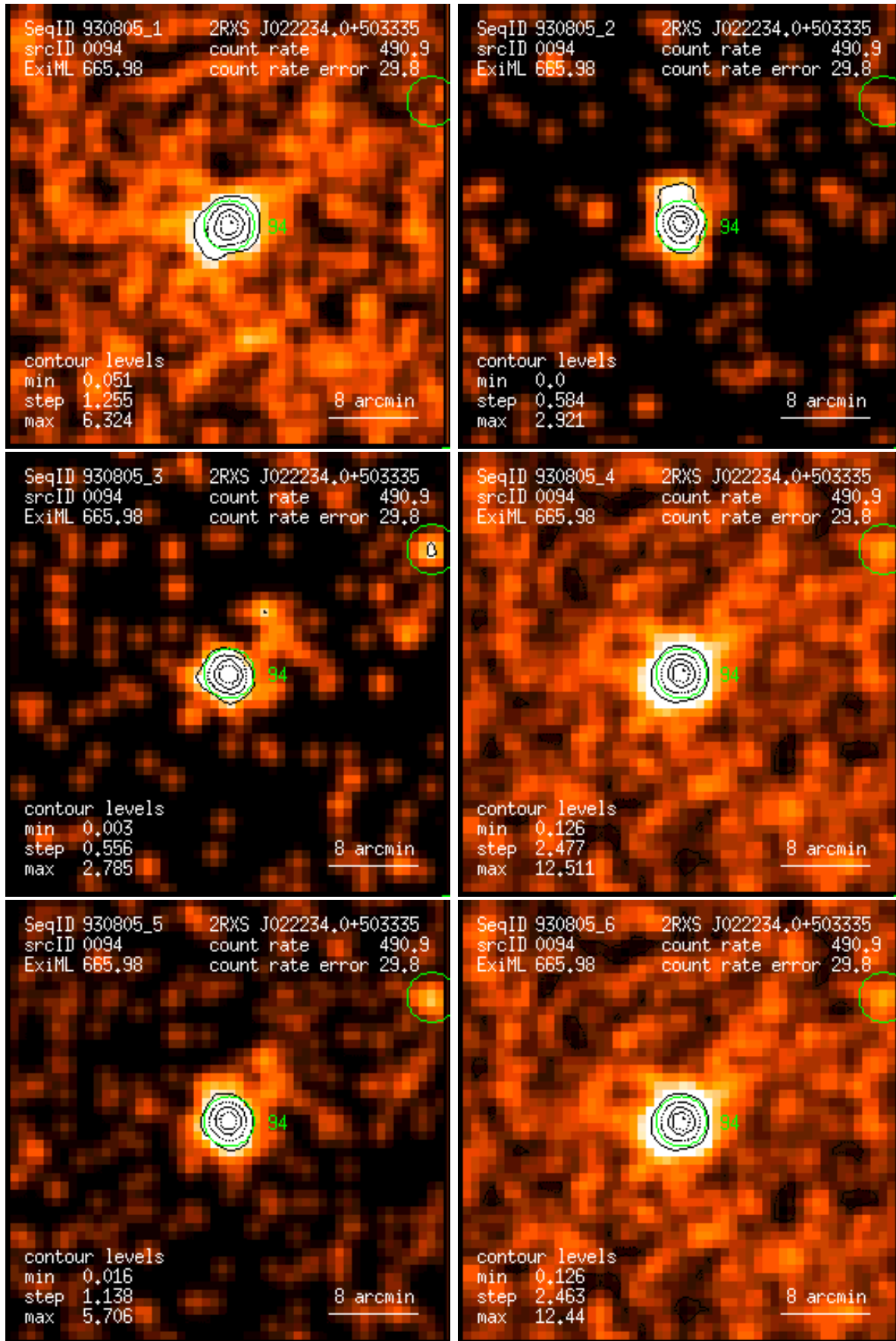
Figure 94: RASS 930805: detection 0094: band rate images, Gaussian filter: (1) PSPC channels 11 – 41, (2) 52 – 90, (3) 91 – 201, (4) 11 – 235, (5) 52 – 201, (6) 11 – 201. Broad band rates in counts/ks. Band rate contour levels in counts/ks/arcmin 2 .
