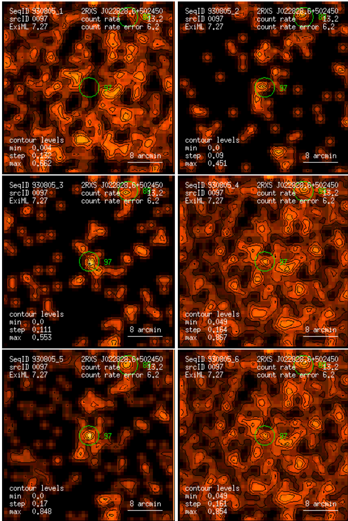
Figure 97: RASS 930805: detection 0097: band rate images, Gaussian filter: (1) PSPC channels 11 – 41, (2) 52 – 90, (3) 91 – 201, (4) 11 – 235, (5) 52 – 201, (6) 11 – 201. Broad band rates in counts/ks. Band rate contour levels in counts/ks/arcmin 2 .
