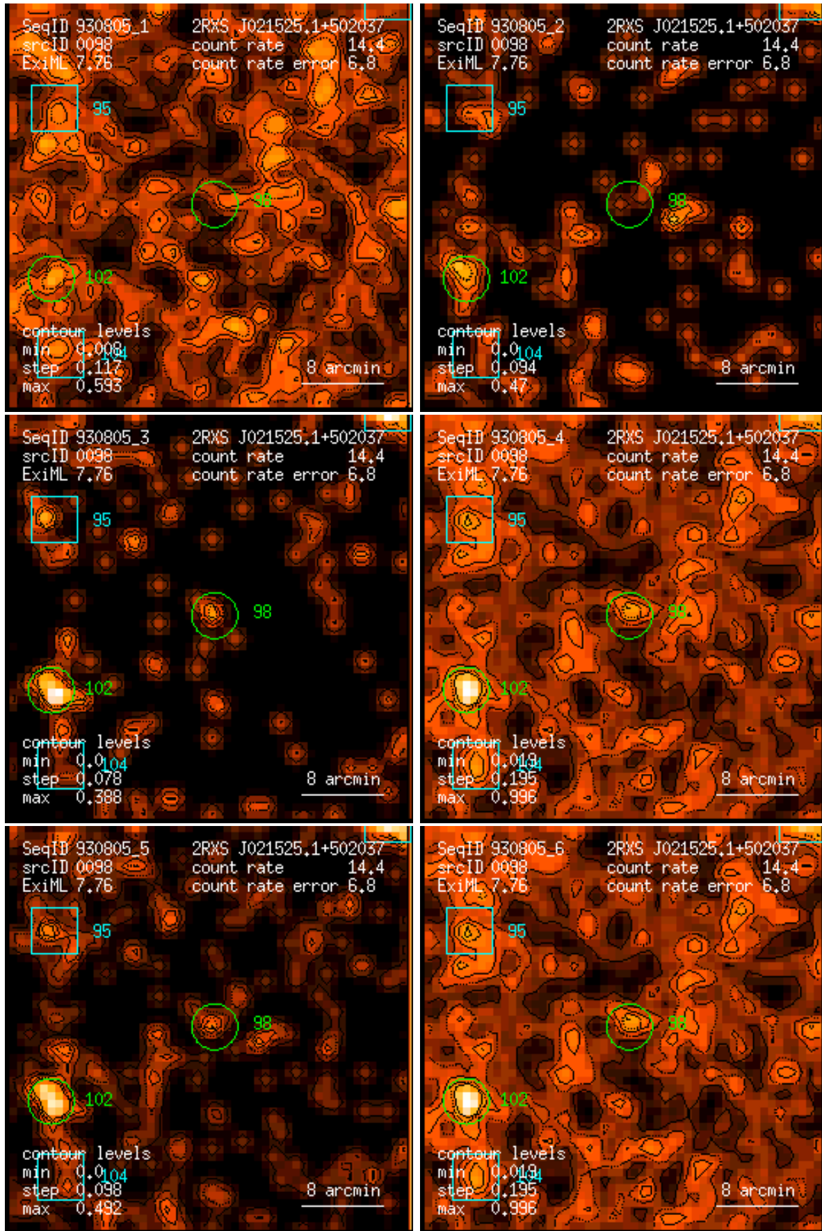
Figure 98: RASS 930805: detection 0098: band rate images, Gaussian filter: (1) PSPC channels 11 – 41, (2) 52 – 90, (3) 91 – 201, (4) 11 – 235, (5) 52 – 201, (6) 11 – 201. Broad band rates in counts/ks. Band rate contour levels in counts/ks/arcmin 2 .
