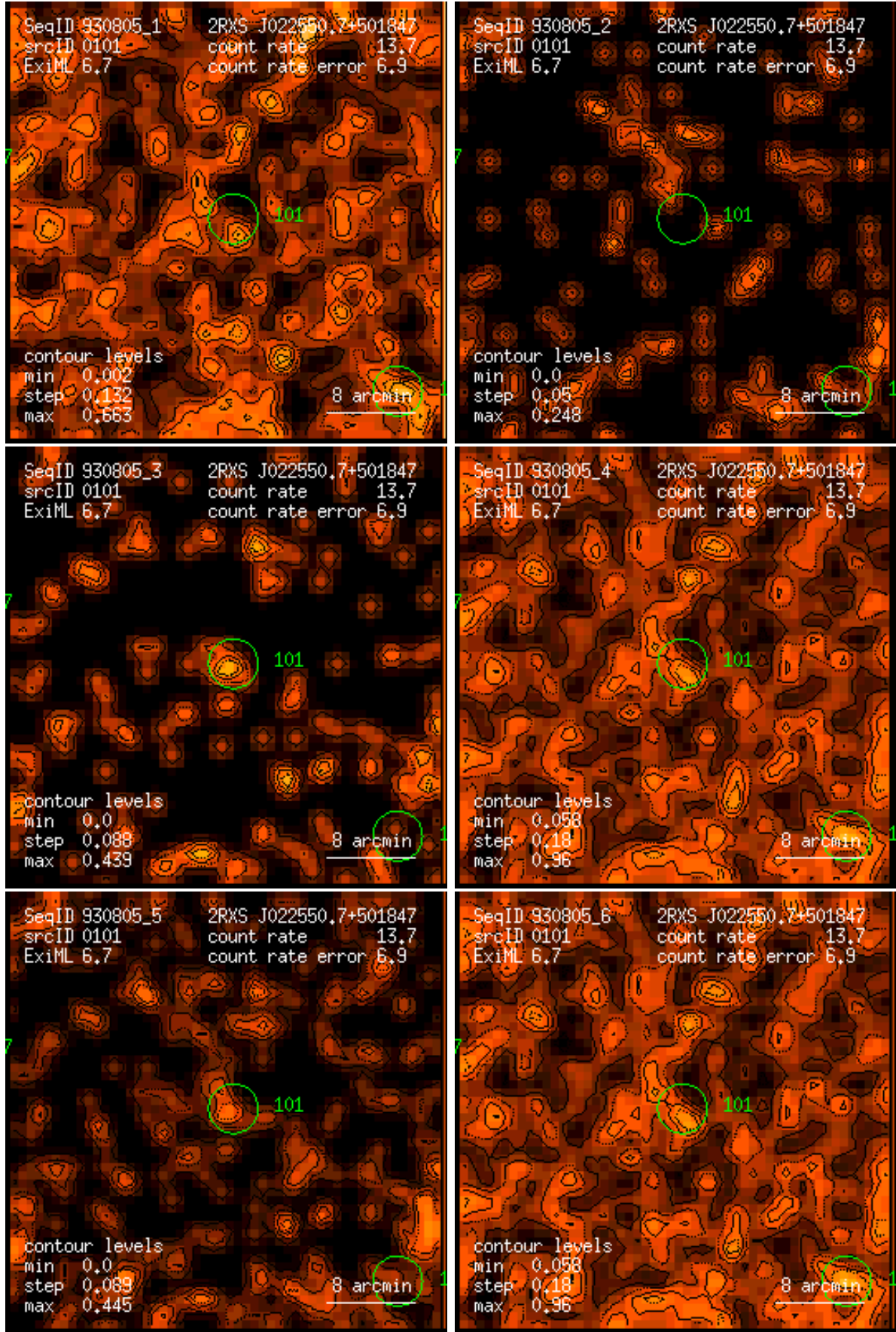
Figure 101: RASS 930805: detection 0101: band rate images, Gaussian filter: (1) PSPC channels 11 – 41, (2) 52 – 90, (3) 91 – 201, (4) 11 – 235, (5) 52 – 201, (6) 11 – 201. Broad band rates in counts/ks. Band rate contour levels in counts/ks/arcmin 2 .
