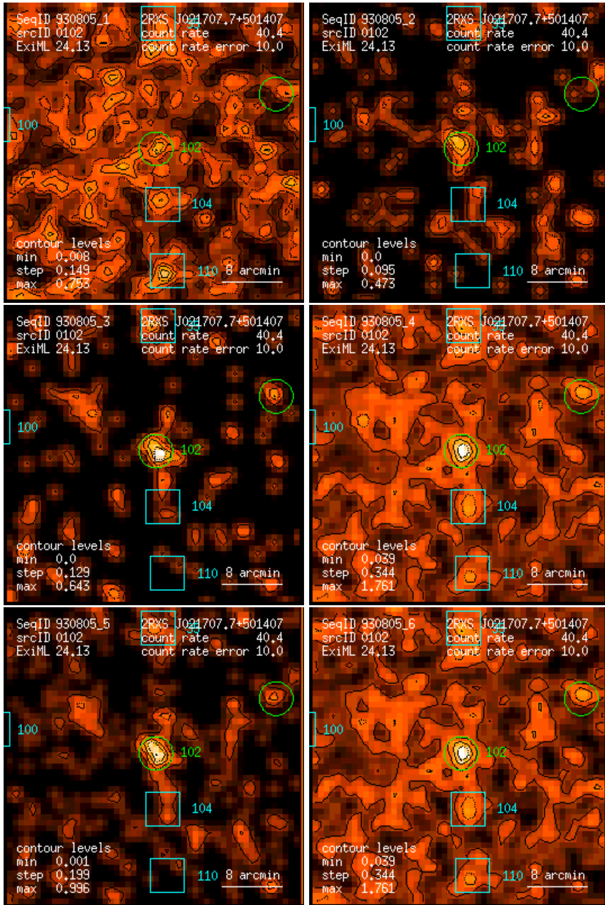
Figure 102: RASS 930805: detection 0102: band rate images, Gaussian filter: (1) PSPC channels 11 – 41, (2) 52 – 90, (3) 91 – 201, (4) 11 – 235, (5) 52 – 201, (6) 11 – 201. Broad band rates in counts/ks. Band rate contour levels in counts/ks/arcmin 2 .
