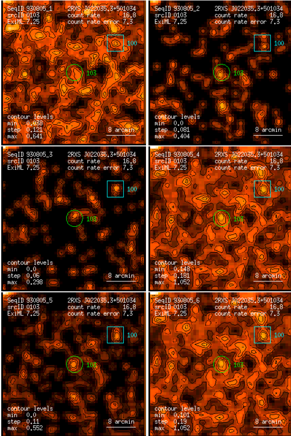
Figure 103: RASS 930805: detection 0103: band rate images, Gaussian filter: (1) PSPC channels 11 – 41, (2) 52 – 90, (3) 91 – 201, (4) 11 – 235, (5) 52 – 201, (6) 11 – 201. Broad band rates in counts/ks. Band rate contour levels in counts/ks/arcmin 2 .
