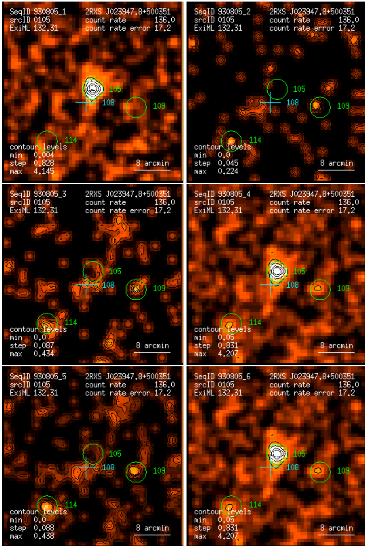
Figure 105: RASS 930805: detection 0105: band rate images, Gaussian filter: (1) PSPC channels 11 – 41, (2) 52 – 90, (3) 91 – 201, (4) 11 – 235, (5) 52 – 201, (6) 11 – 201. Broad band rates in counts/ks. Band rate contour levels in counts/ks/arcmin 2 .
