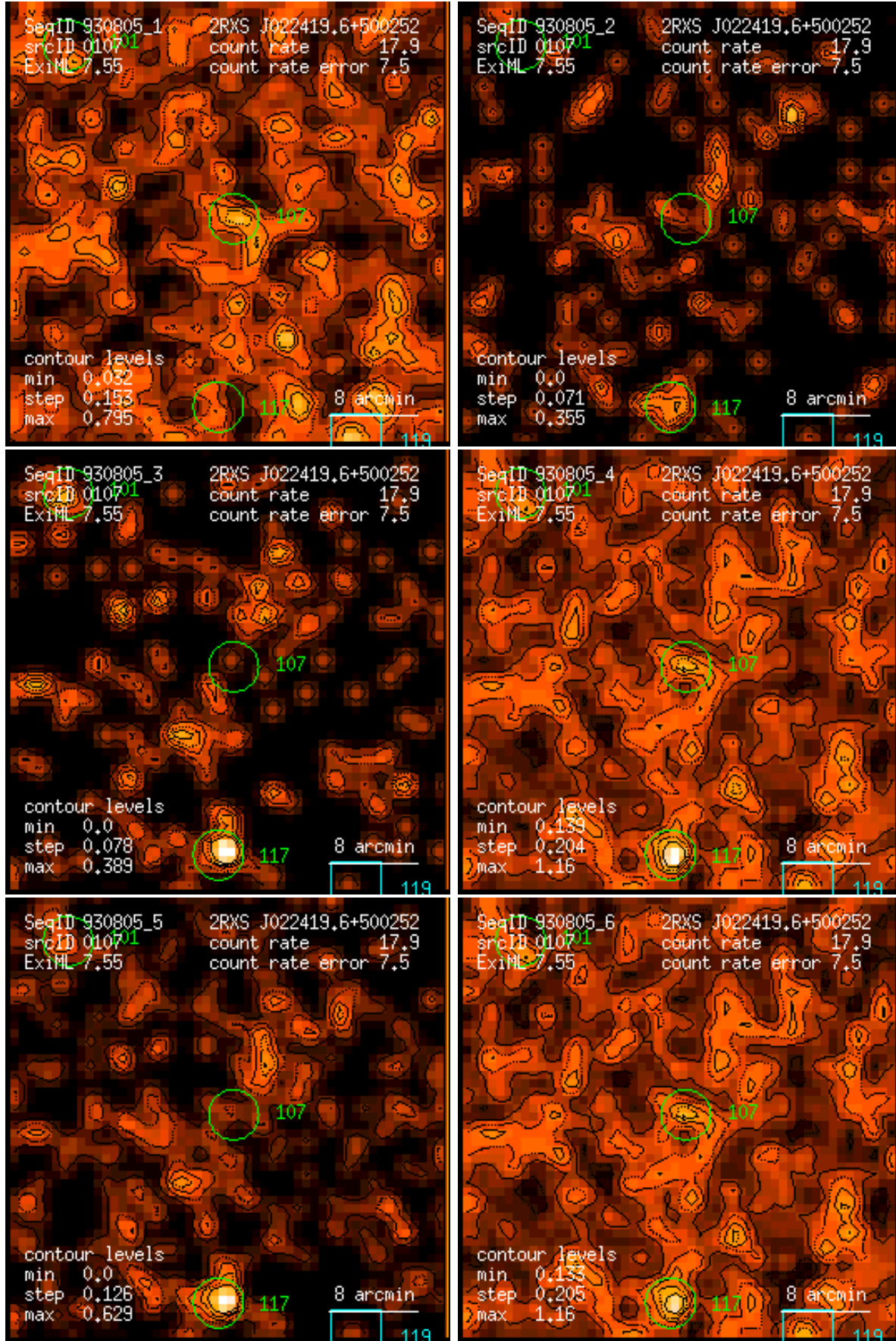
Figure 107: RASS 930805: detection 0107: band rate images, Gaussian filter: (1) PSPC channels 11 – 41, (2) 52 – 90, (3) 91 – 201, (4) 11 – 235, (5) 52 – 201, (6) 11 – 201. Broad band rates in counts/ks. Band rate contour levels in counts/ks/arcmin 2 .
