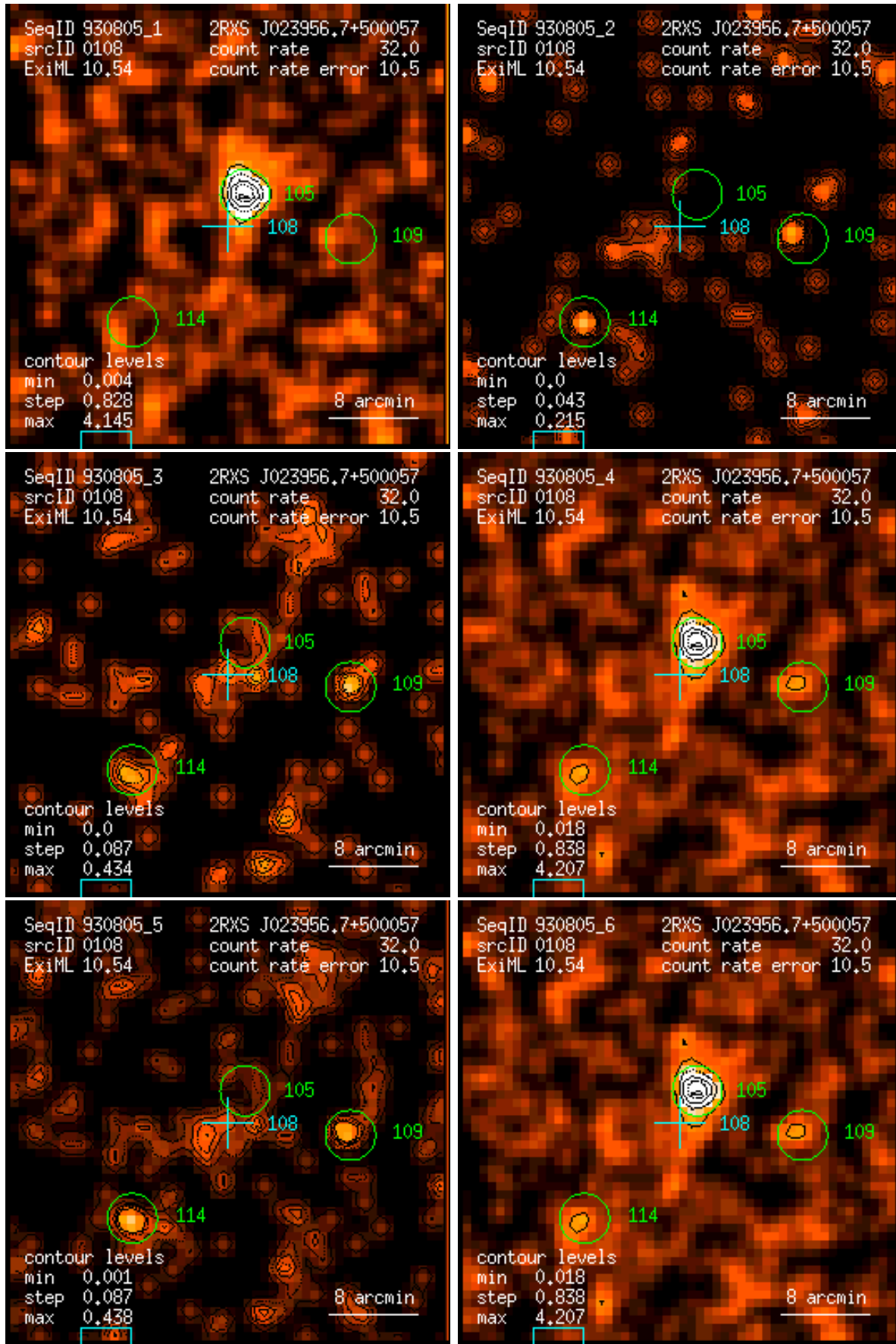
Figure 108: RASS 930805: detection 0108: band rate images, Gaussian filter: (1) PSPC channels 11 – 41, (2) 52 – 90, (3) 91 – 201, (4) 11 – 235, (5) 52 – 201, (6) 11 – 201. Broad band rates in counts/ks. Band rate contour levels in counts/ks/arcmin 2 .
