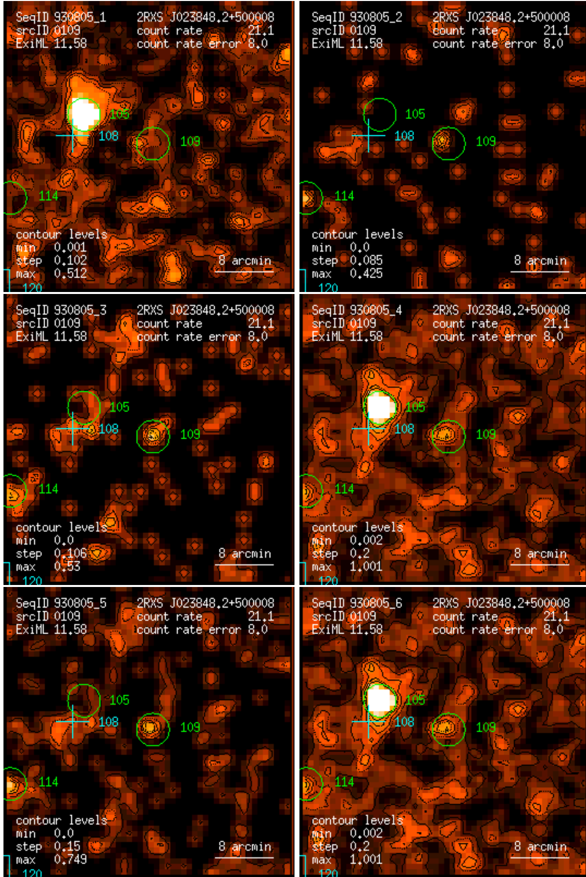
Figure 109: RASS 930805: detection 0109: band rate images, Gaussian filter: (1) PSPC channels 11 – 41, (2) 52 – 90, (3) 91 – 201, (4) 11 – 235, (5) 52 – 201, (6) 11 – 201. Broad band rates in counts/ks. Band rate contour levels in counts/ks/arcmin 2 .
