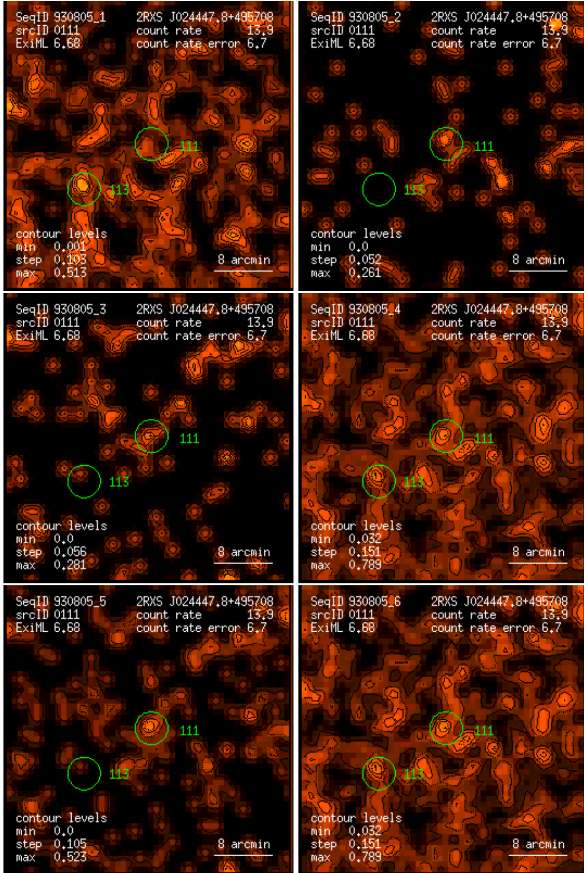
Figure 111: RASS 930805: detection 0111: band rate images, Gaussian filter: (1) PSPC channels 11 – 41, (2) 52 – 90, (3) 91 – 201, (4) 11 – 235, (5) 52 – 201, (6) 11 – 201. Broad band rates in counts/ks. Band rate contour levels in counts/ks/arcmin 2 .
