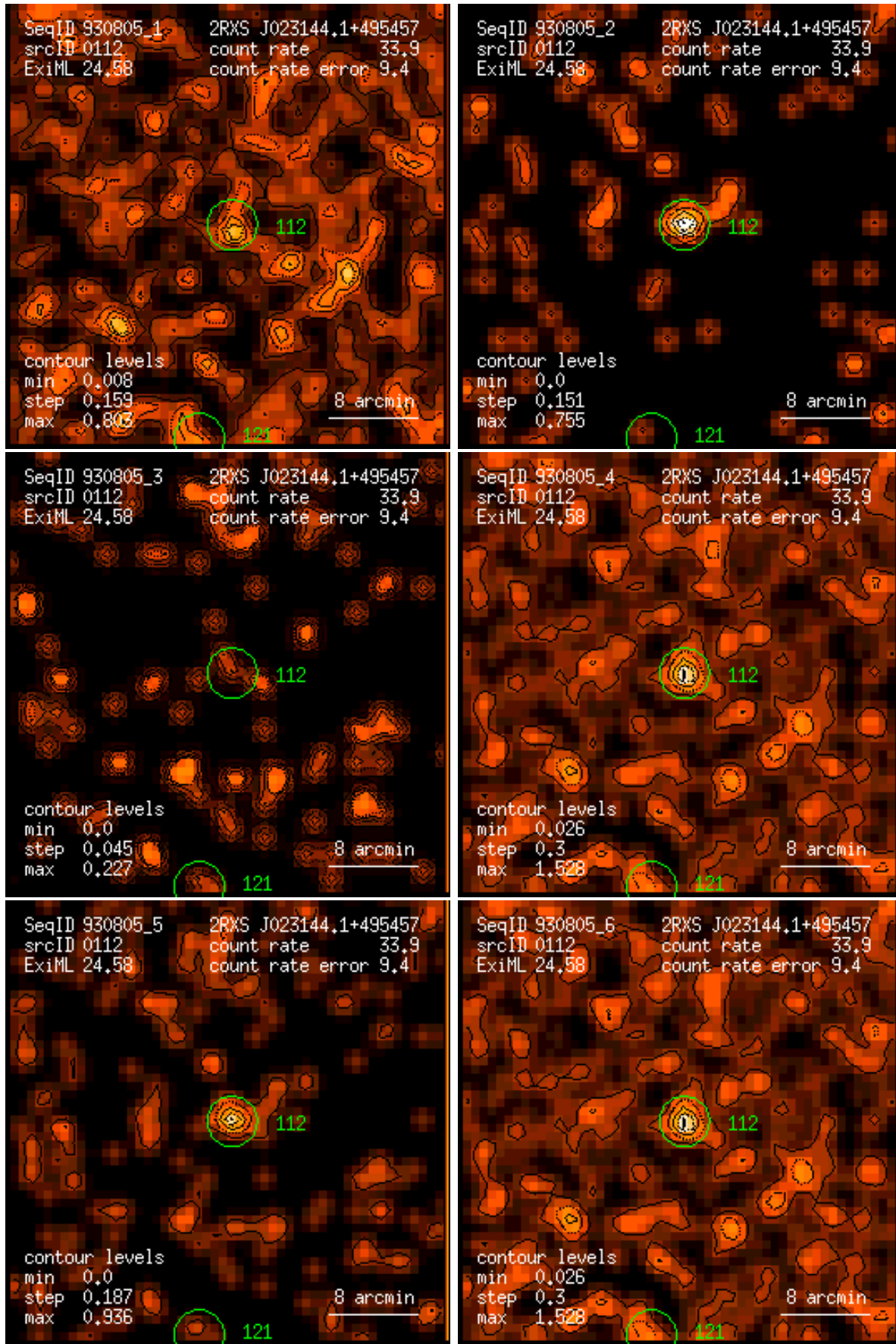
Figure 112: RASS 930805: detection 0112: band rate images, Gaussian filter: (1) PSPC channels 11 – 41, (2) 52 – 90, (3) 91 – 201, (4) 11 – 235, (5) 52 – 201, (6) 11 – 201. Broad band rates in counts/ks. Band rate contour levels in counts/ks/arcmin 2 .
