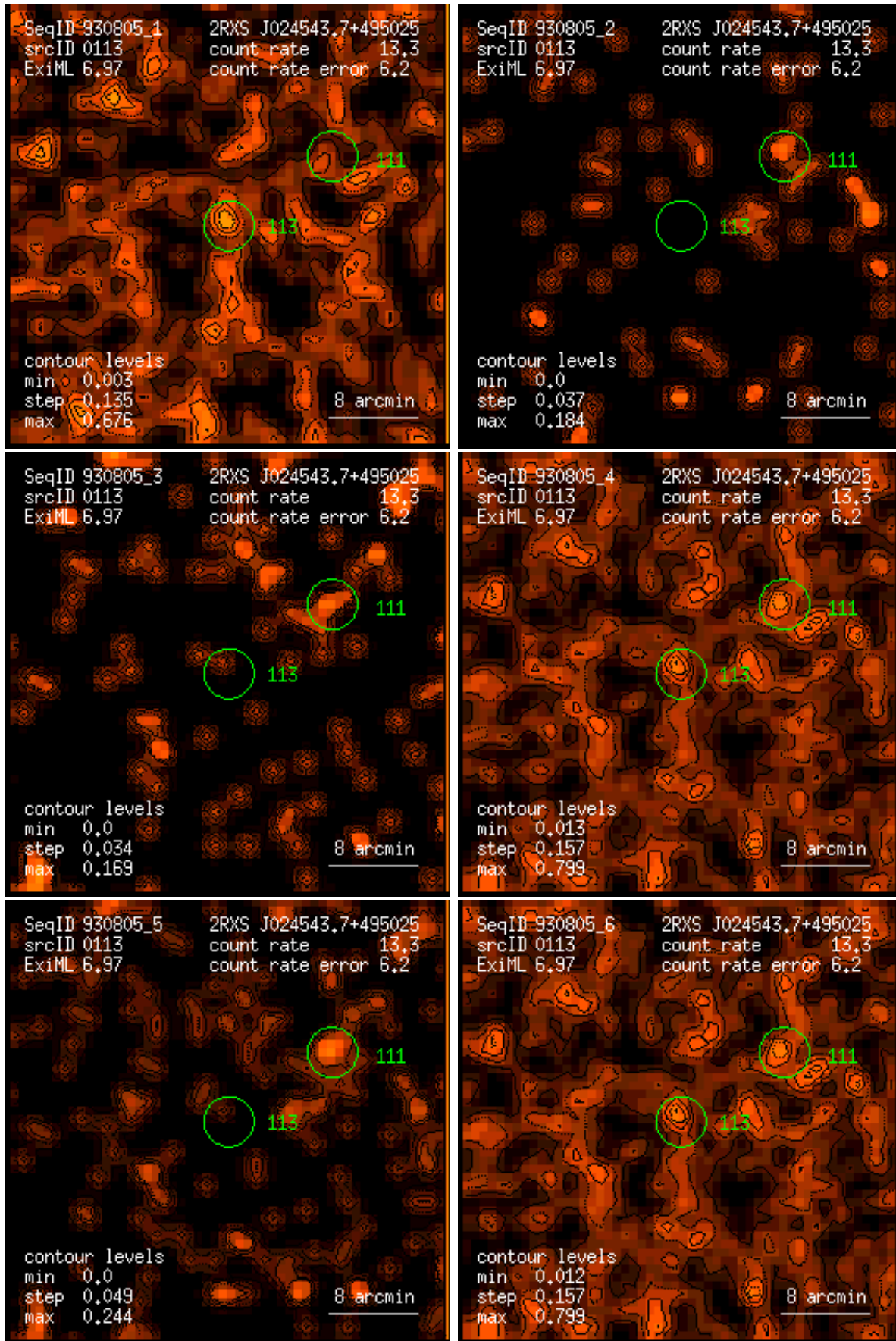
Figure 113: RASS 930805: detection 0113: band rate images, Gaussian filter: (1) PSPC channels 11 – 41, (2) 52 – 90, (3) 91 – 201, (4) 11 – 235, (5) 52 – 201, (6) 11 – 201. Broad band rates in counts/ks. Band rate contour levels in counts/ks/arcmin 2 .
