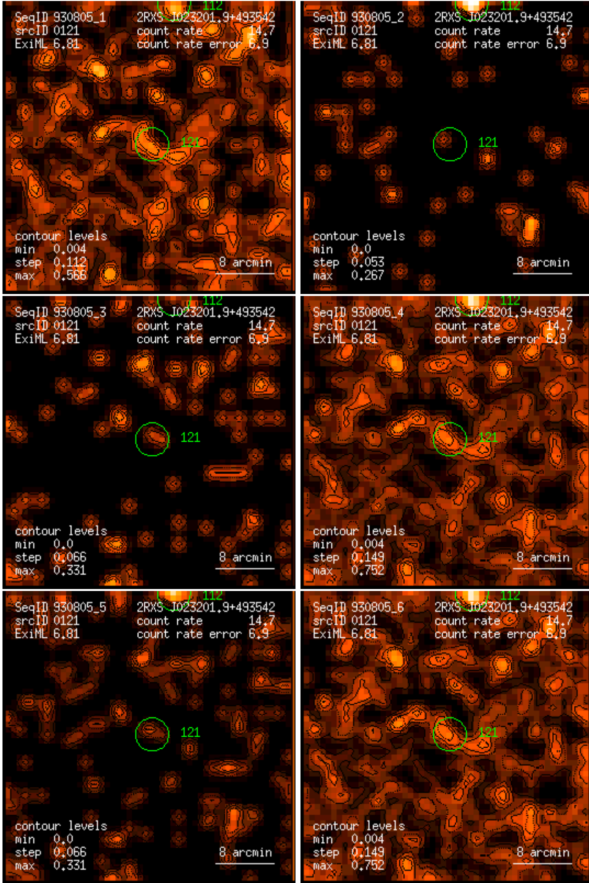
Figure 121: RASS 930805: detection 0121: band rate images, Gaussian filter: (1) PSPC channels 11 – 41, (2) 52 – 90, (3) 91 – 201, (4) 11 – 235, (5) 52 – 201, (6) 11 – 201. Broad band rates in counts/ks. Band rate contour levels in counts/ks/arcmin 2 .
