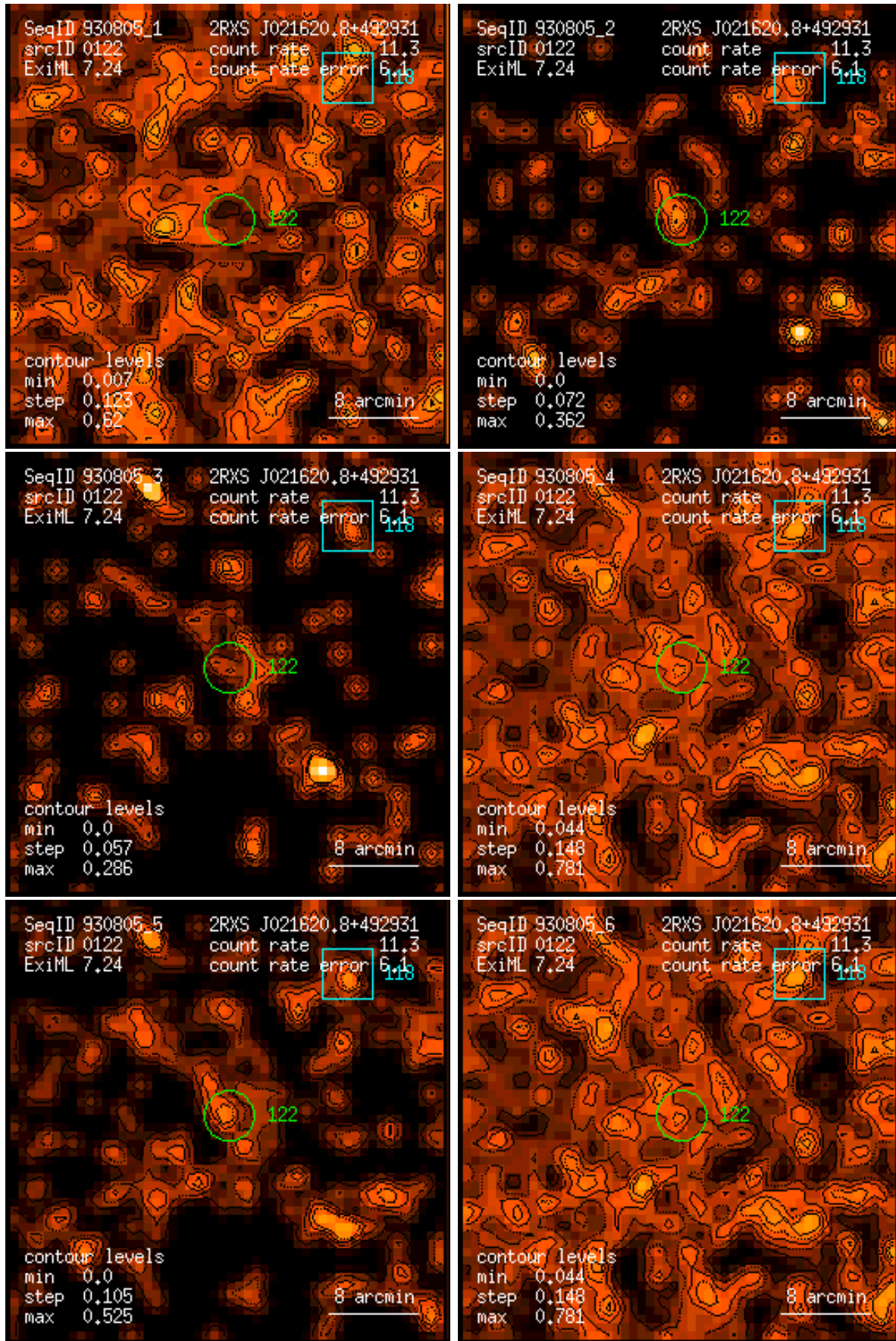
Figure 122: RASS 930805: detection 0122: band rate images, Gaussian filter: (1) PSPC channels 11 – 41, (2) 52 – 90, (3) 91 – 201, (4) 11 – 235, (5) 52 – 201, (6) 11 – 201. Broad band rates in counts/ks. Band rate contour levels in counts/ks/arcmin 2 .
