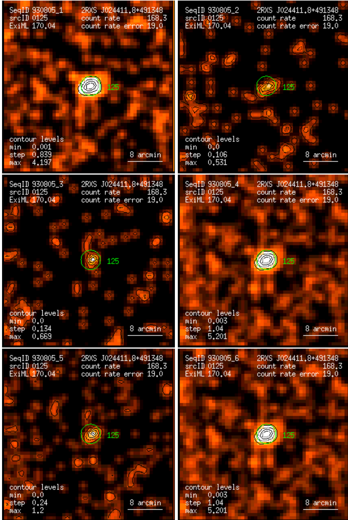
Figure 125: RASS 930805: detection 0125: band rate images, Gaussian filter: (1) PSPC channels 11 – 41, (2) 52 – 90, (3) 91 – 201, (4) 11 – 235, (5) 52 – 201, (6) 11 – 201. Broad band rates in counts/ks. Band rate contour levels in counts/ks/arcmin 2 .
