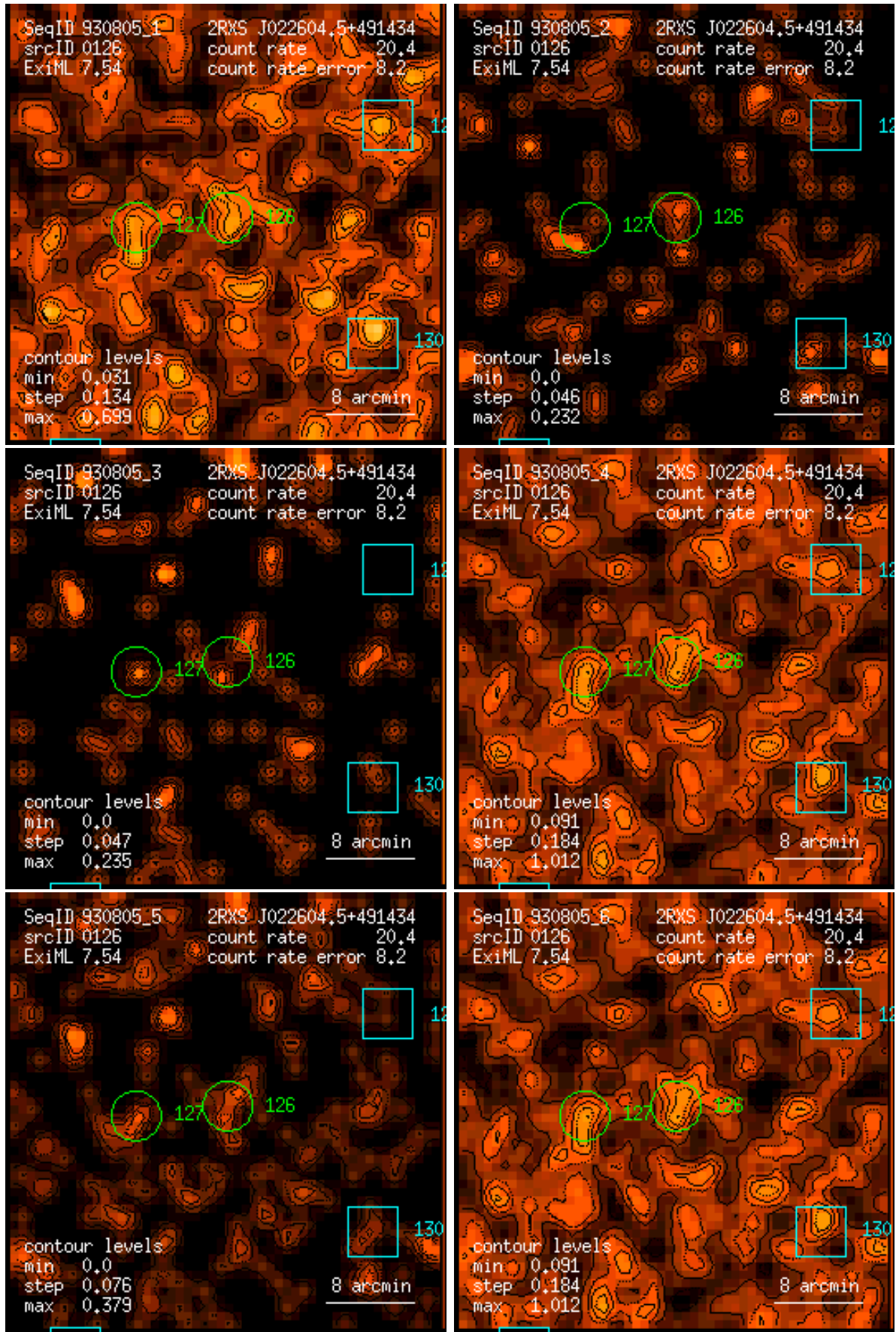
Figure 126: RASS 930805: detection 0126: band rate images, Gaussian filter: (1) PSPC channels 11 – 41, (2) 52 – 90, (3) 91 – 201, (4) 11 – 235, (5) 52 – 201, (6) 11 – 201. Broad band rates in counts/ks. Band rate contour levels in counts/ks/arcmin 2 .
