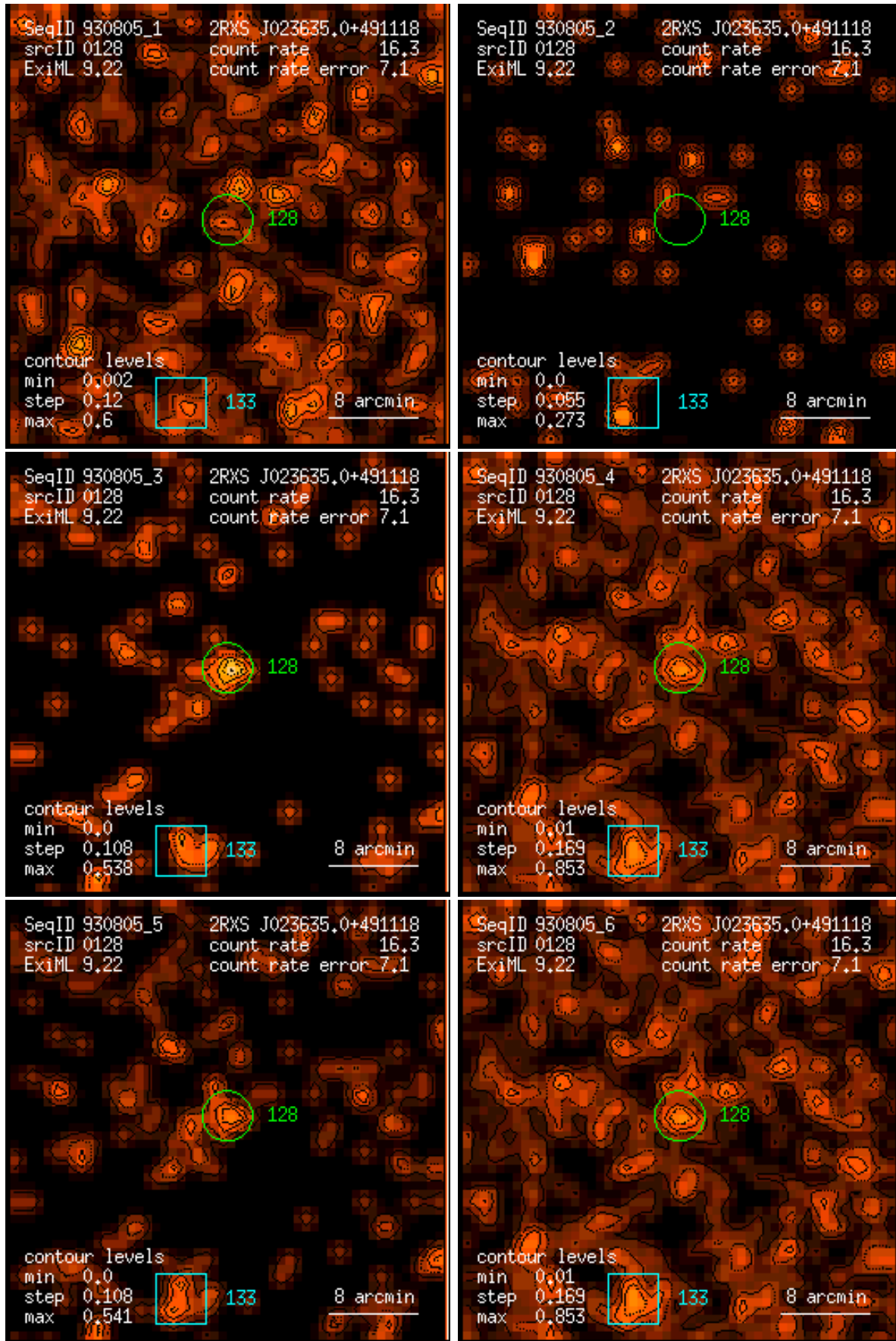
Figure 128: RASS 930805: detection 0128: band rate images, Gaussian filter: (1) PSPC channels 11 – 41, (2) 52 – 90, (3) 91 – 201, (4) 11 – 235, (5) 52 – 201, (6) 11 – 201. Broad band rates in counts/ks. Band rate contour levels in counts/ks/arcmin 2 .
