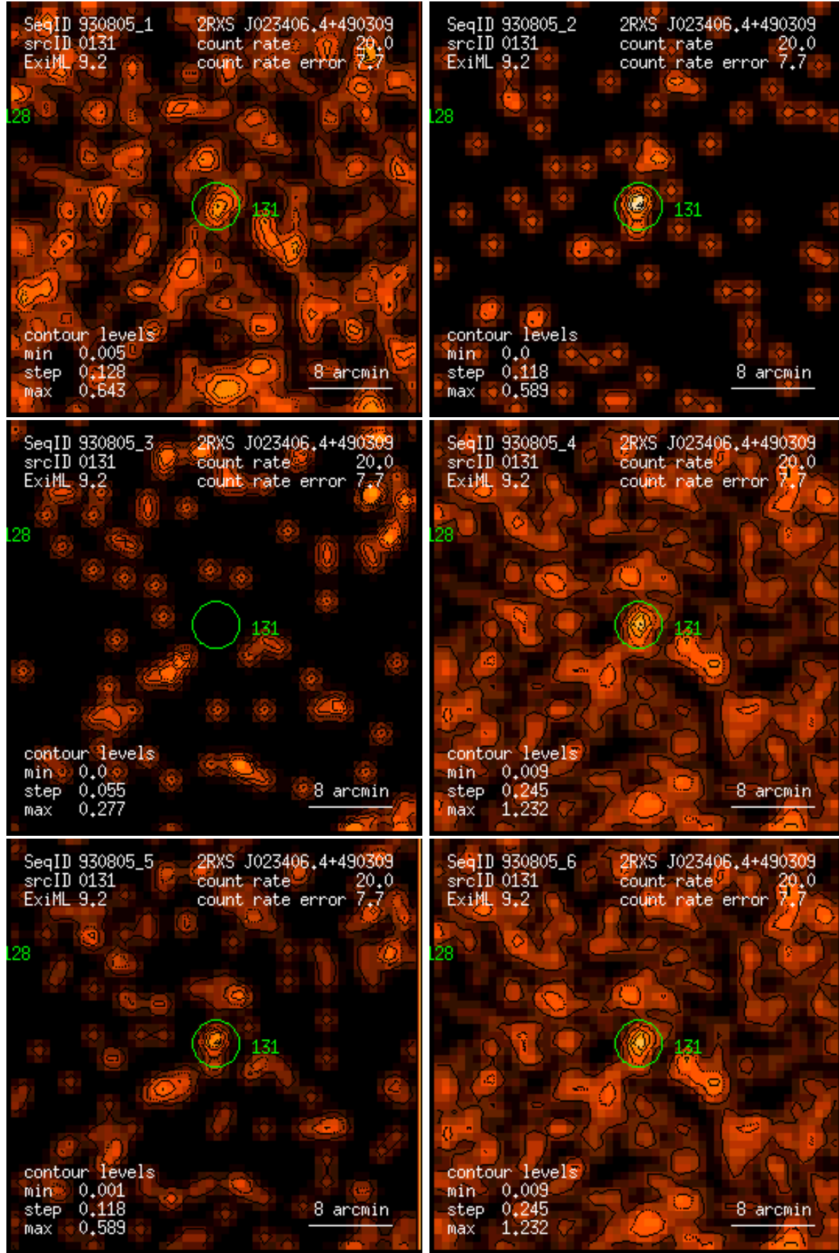
Figure 131: RASS 930805: detection 0131: band rate images, Gaussian filter: (1) PSPC channels 11 – 41, (2) 52 – 90, (3) 91 – 201, (4) 11 – 235, (5) 52 – 201, (6) 11 – 201. Broad band rates in counts/ks. Band rate contour levels in counts/ks/arcmin 2 .
