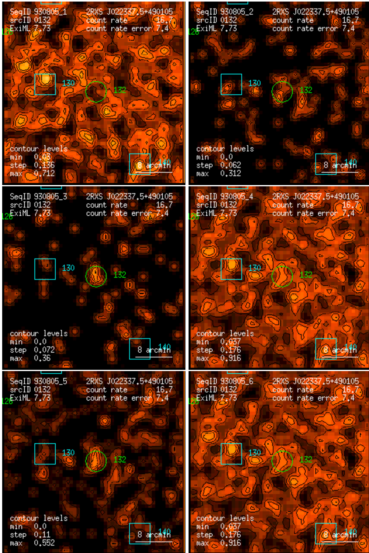
Figure 132: RASS 930805: detection 0132: band rate images, Gaussian filter: (1) PSPC channels 11 – 41, (2) 52 – 90, (3) 91 – 201, (4) 11 – 235, (5) 52 – 201, (6) 11 – 201. Broad band rates in counts/ks. Band rate contour levels in counts/ks/arcmin 2 .
