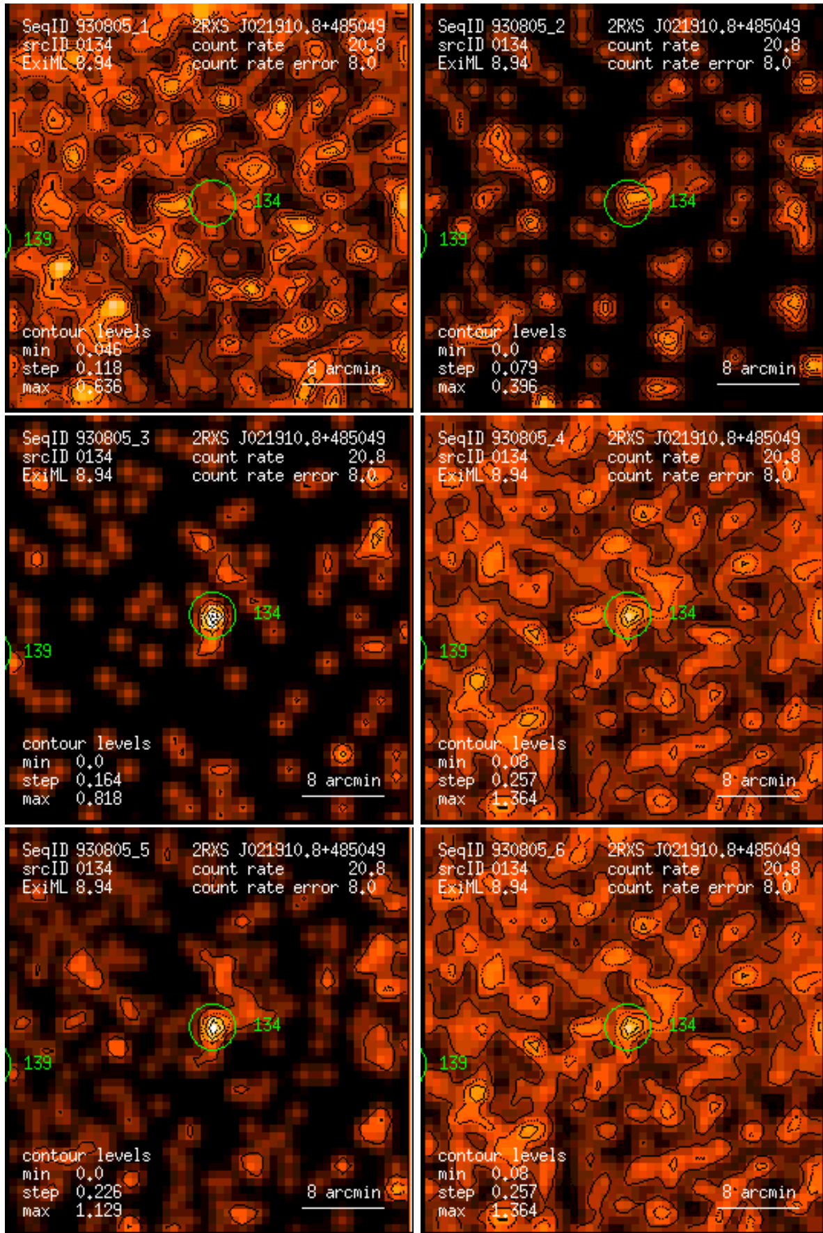
Figure 134: RASS 930805: detection 0134: band rate images, Gaussian filter: (1) PSPC channels 11 – 41, (2) 52 – 90, (3) 91 – 201, (4) 11 – 235, (5) 52 – 201, (6) 11 – 201. Broad band rates in counts/ks. Band rate contour levels in counts/ks/arcmin 2 .
